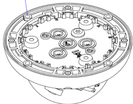
Mounting ring
