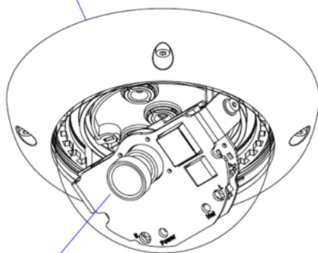
Lens
