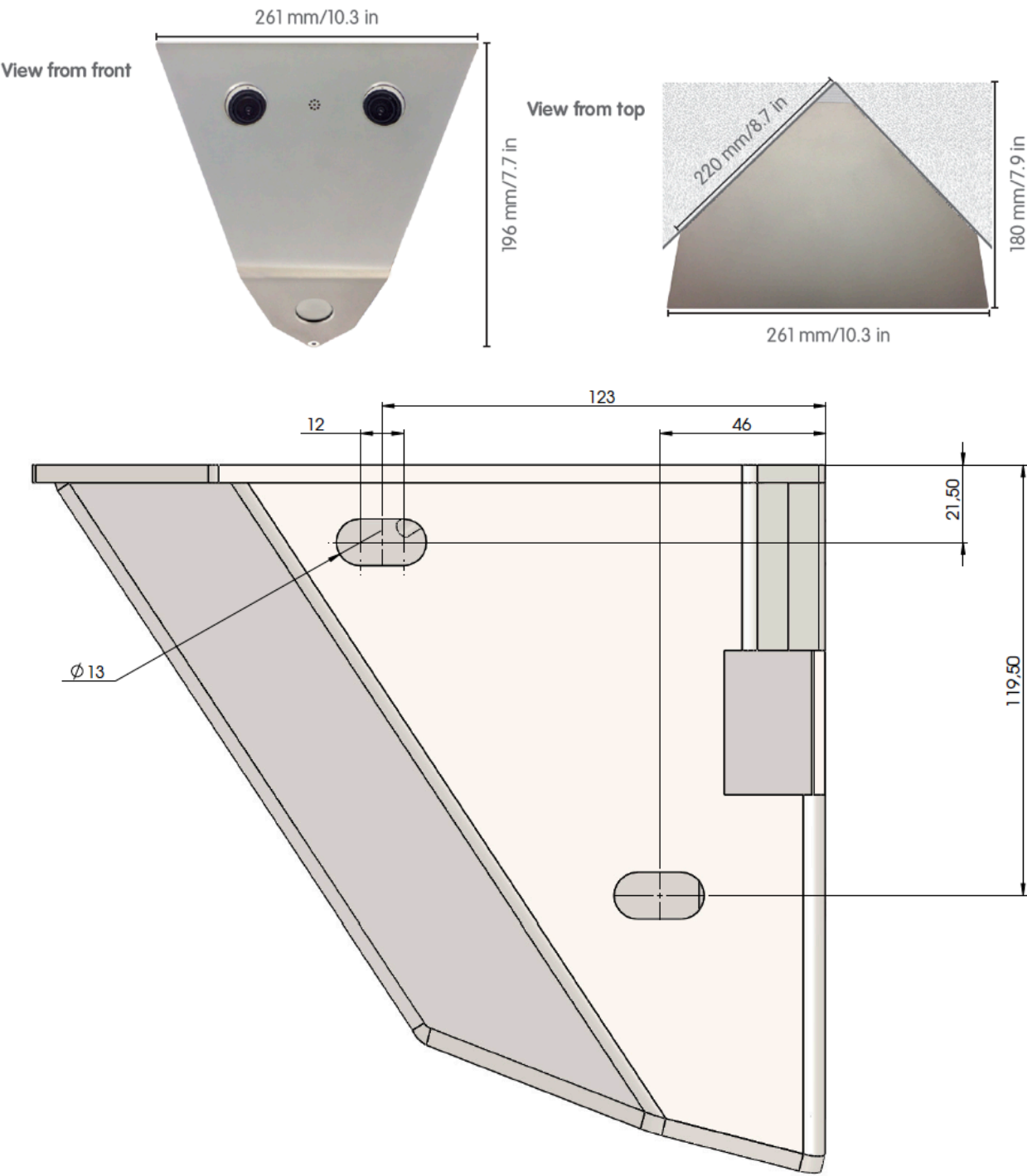
Abmessungen in mm
