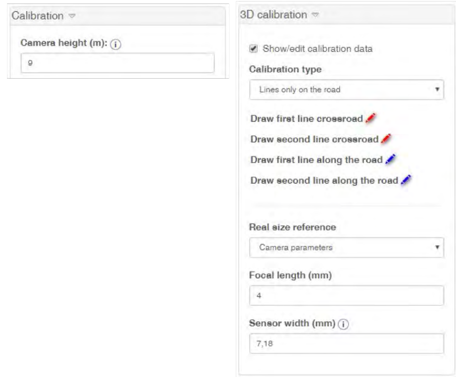
Fig. 69: 3D Calibration for AI-ROAD 3D
