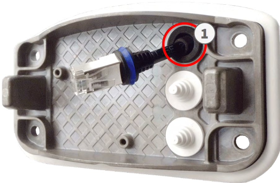
Abb. 34: Prepare the mounting plate
