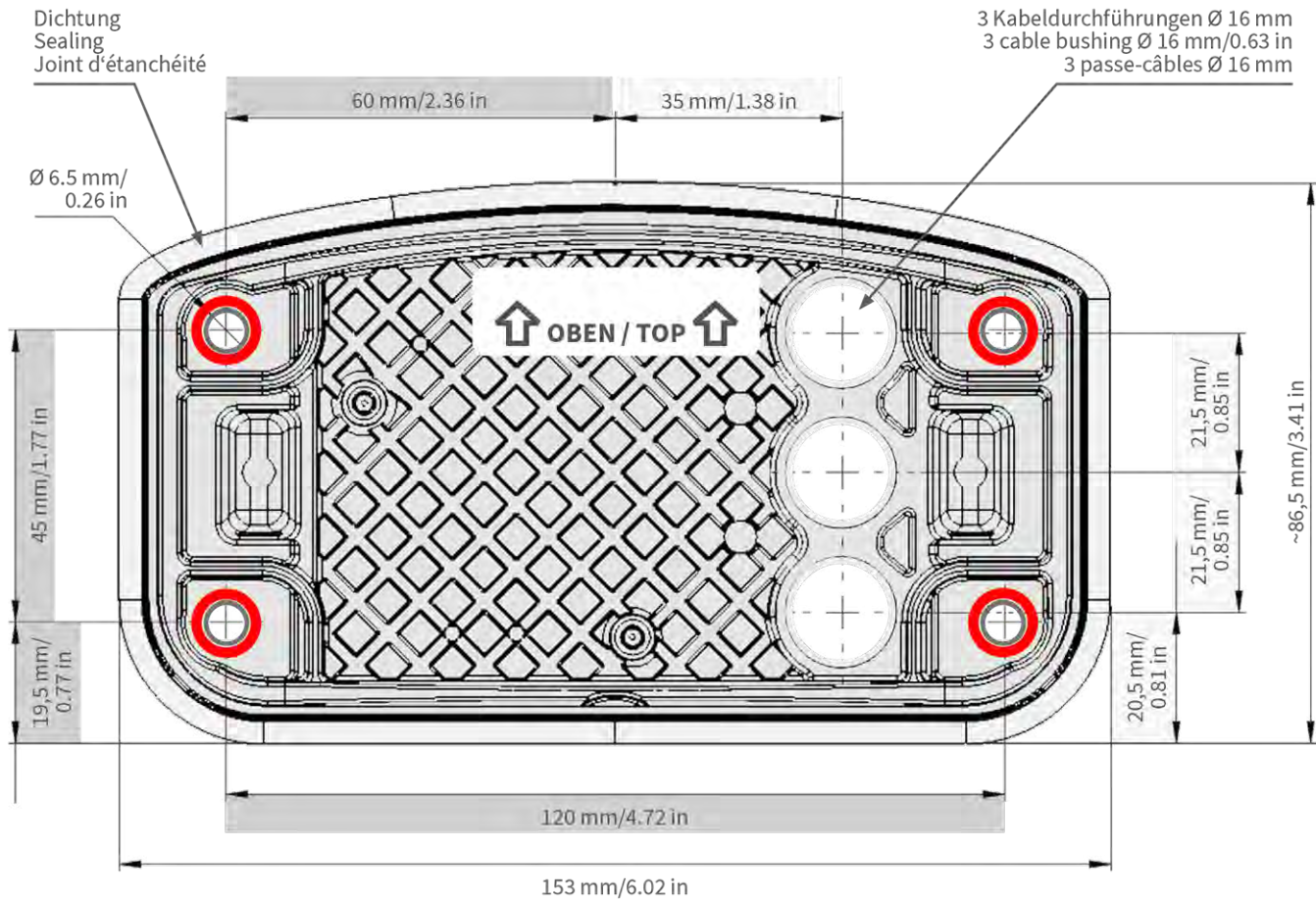
Abb. 32: Mounting plate with holes for positioning the fastener screws
