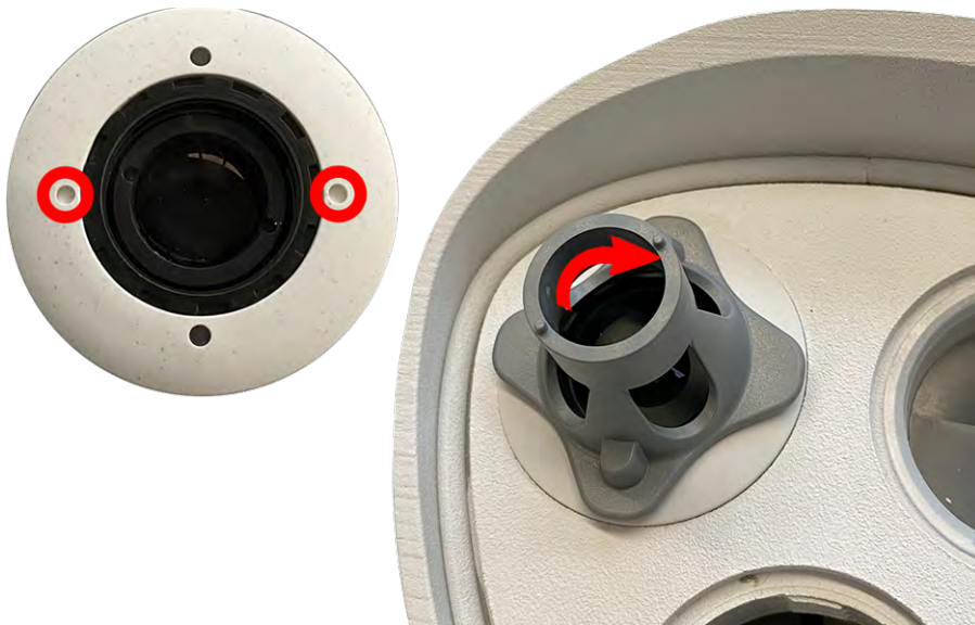
Abb. 30: Lock the sensor module
