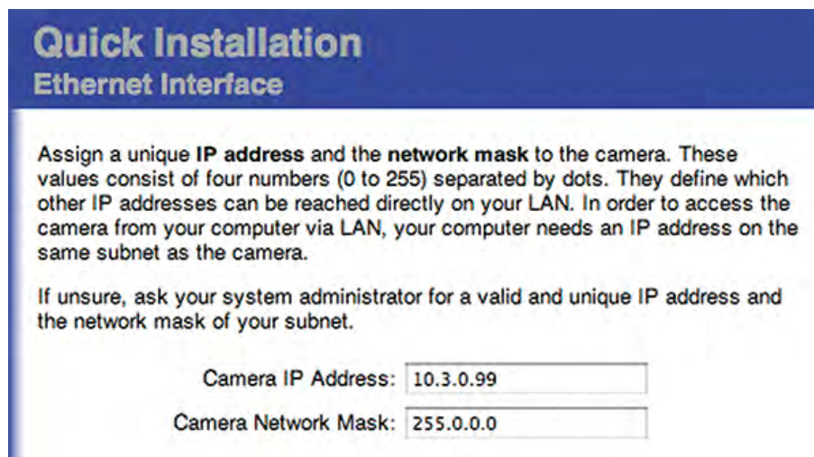
Abb. 50: Network settings in the web interface of the camera
