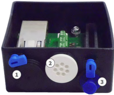
Abb. 37: Connector box with rubber plug Ethernet C.3 (1), rubber plug single-wire C.4 (2), USB plug (3) and two blue locks
