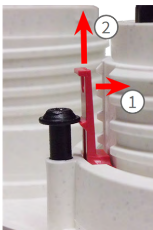
Abb. 21: Remove a security clip
