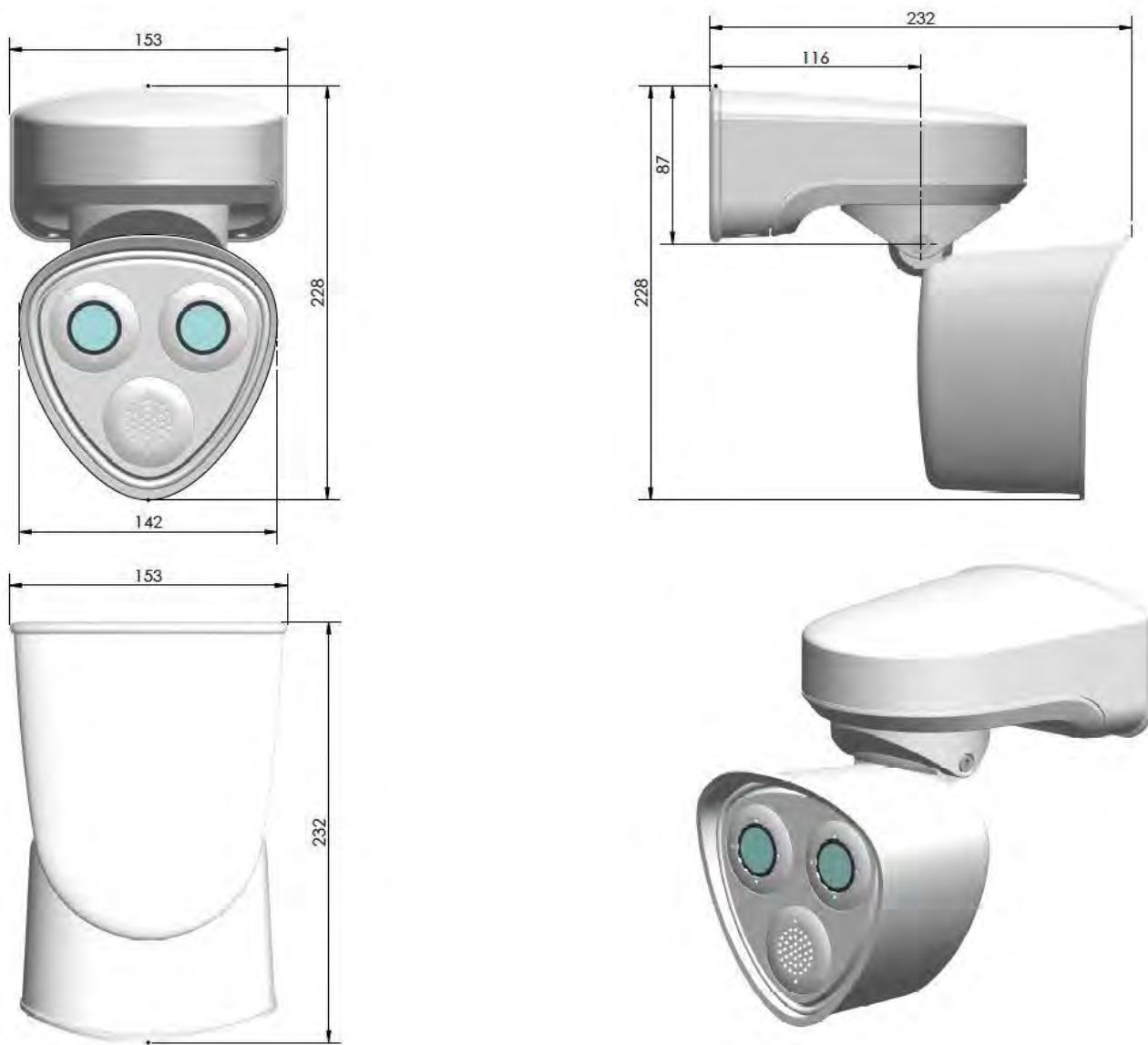
Abb. 4: M73: All measurements in mm
