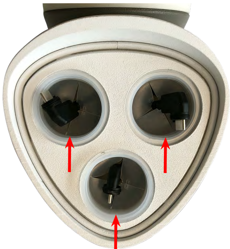
Abb. 7: Remove the transport plugs
