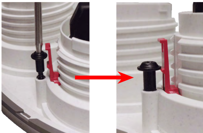
Abb. 17: Use screw to lock security clip in place
