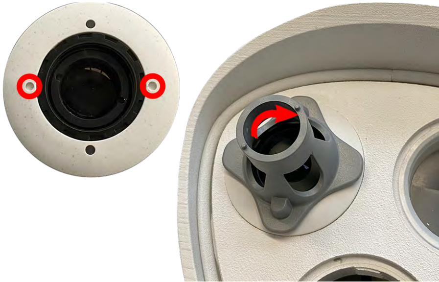
Abb. 11: Lock the sensor module
