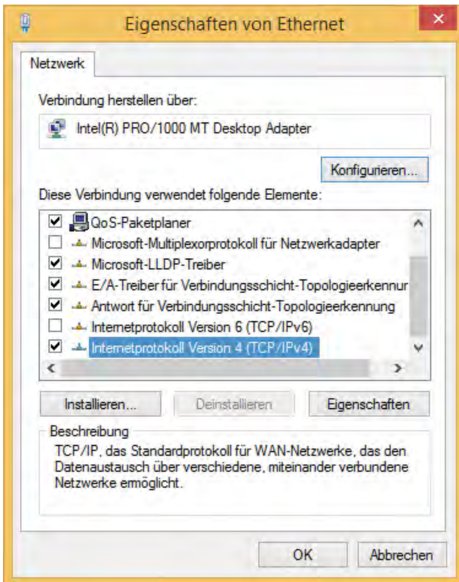
Abb. 47: Network settings on Windows machines
