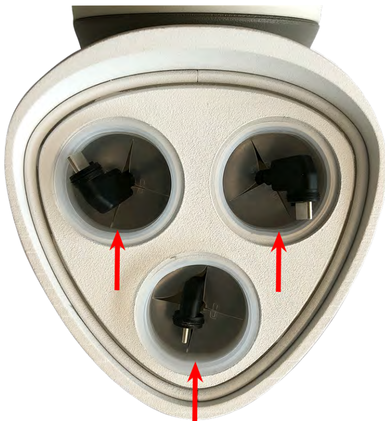
Abb. 26: Remove the transport plugs
