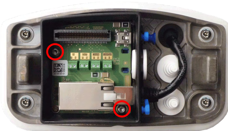
Abb. 39: Mounting the connector box (top view) using the two screws (highlighted red in the figure) on the mounting plate
