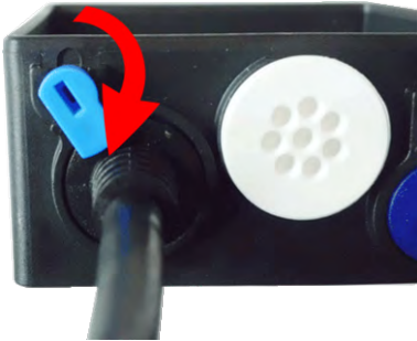
Abb. 38: Lock the network cable in the connector box
