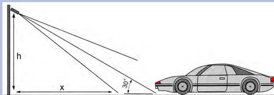
Fig. 9: Vertical pointing of the camera
