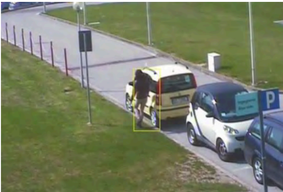
Fig. 46: AI-LOITERING: configuration
