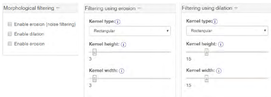
Fig. 13: Morphological filtering
