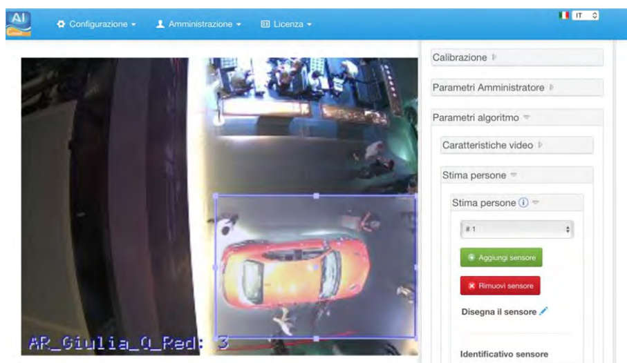
Fig. 64: AI-CROWD: configuration
