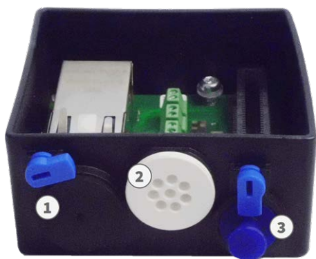
Fig. 46: Connector Box RJ45
