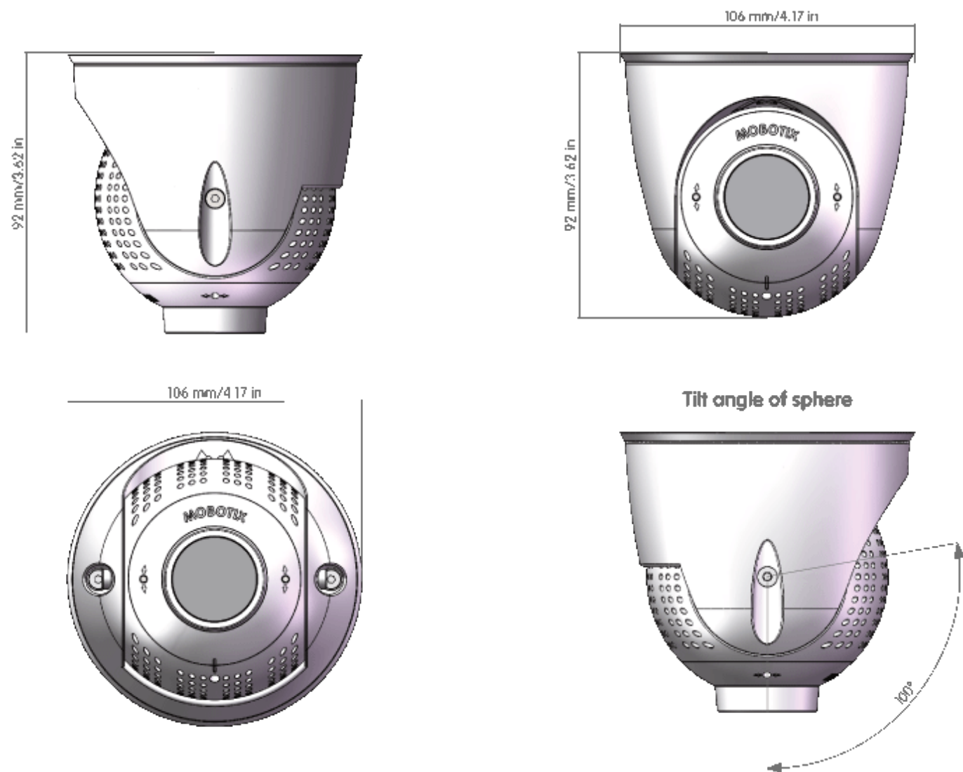
Abb. 7: PTMount-Thermal
