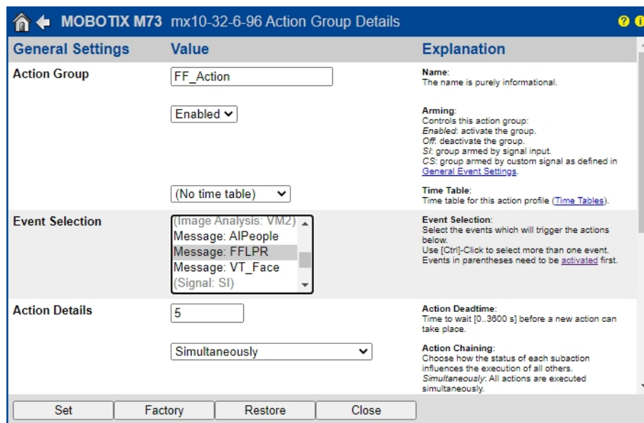
Fig. 26: Configuring an Action Group
