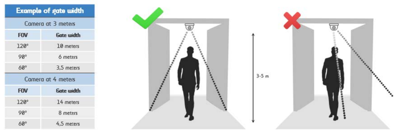
Fig. 60: camera position
