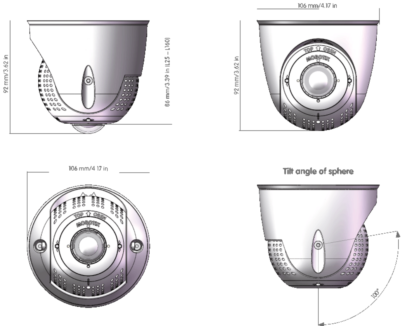
Fig. 6: PTMount
