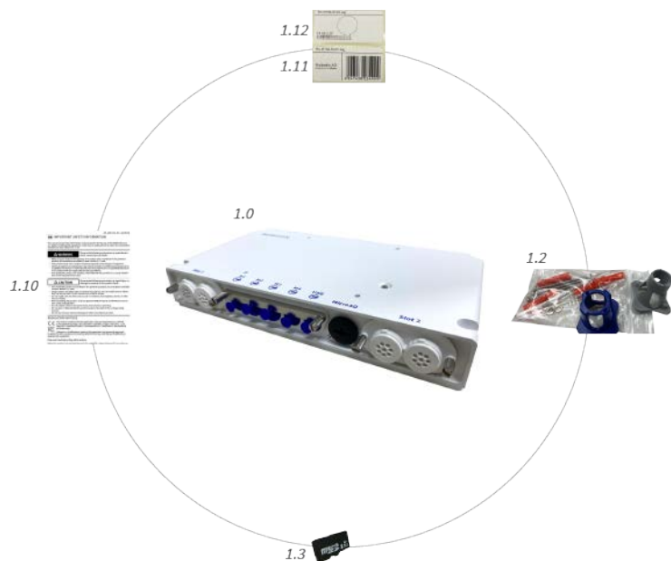
Fig. 1: Scope of delivery S74
