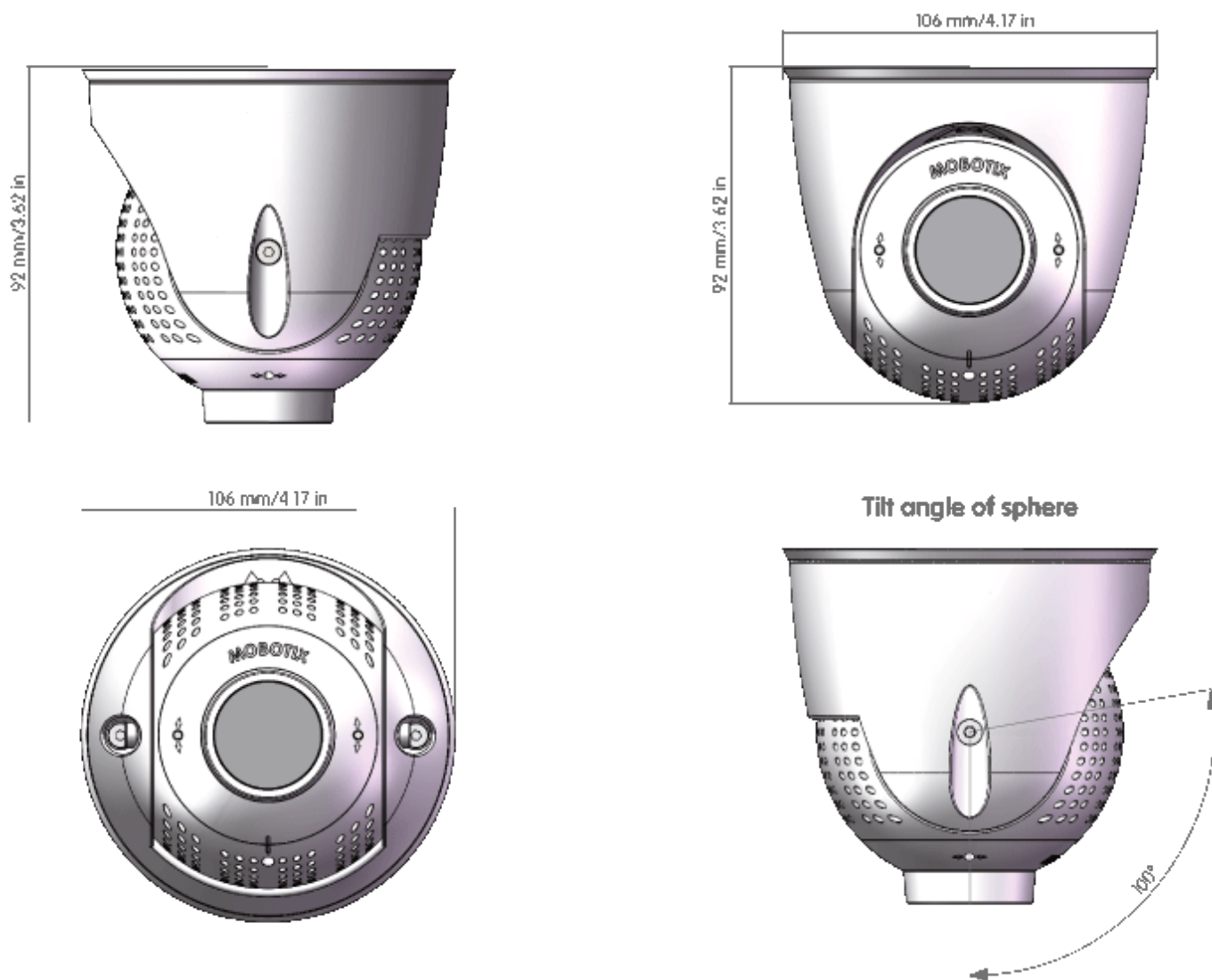
Fig. 7: PTMount-Thermal
