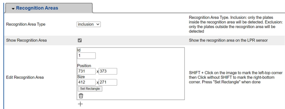
Fig. 13: Recognition Areas
