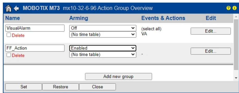
Fig. 25: Defining Action Groups
