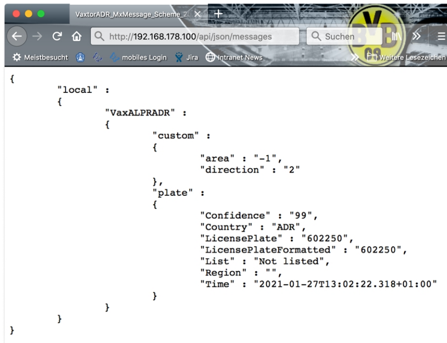
Fig. 26: Example: Meta data transmitted within an MxMessage of the Vaxtor License Plate Recognition / Dangerous Goods App
