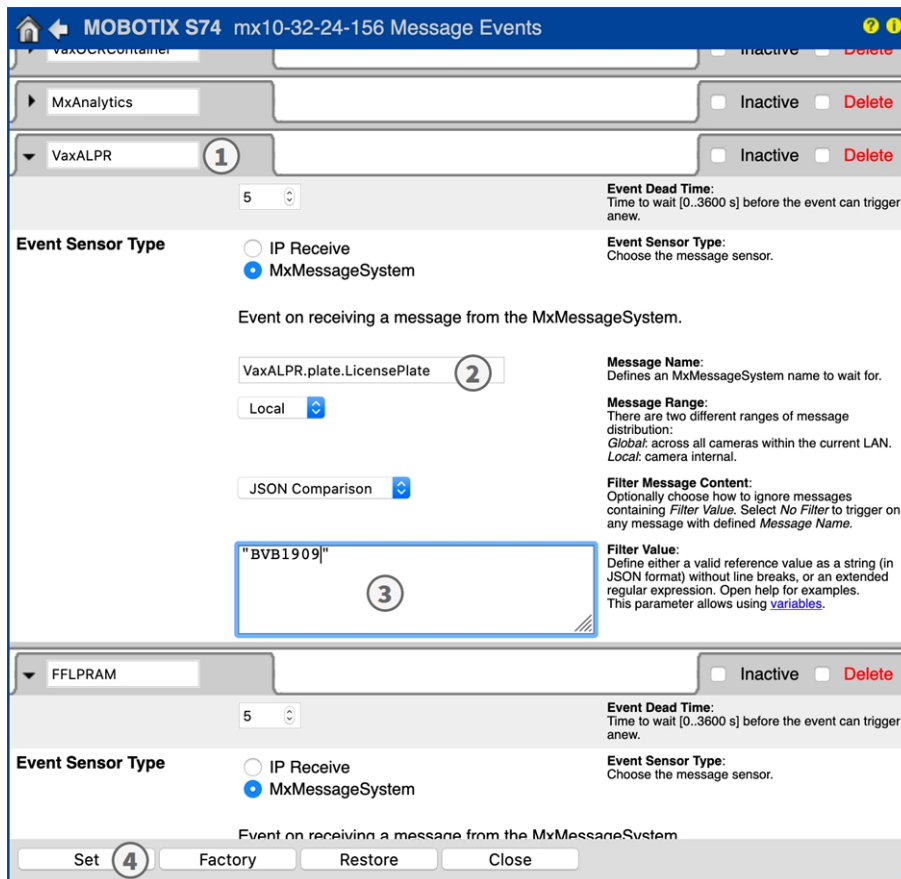
Fig. 30: Example: Unique license plate event
