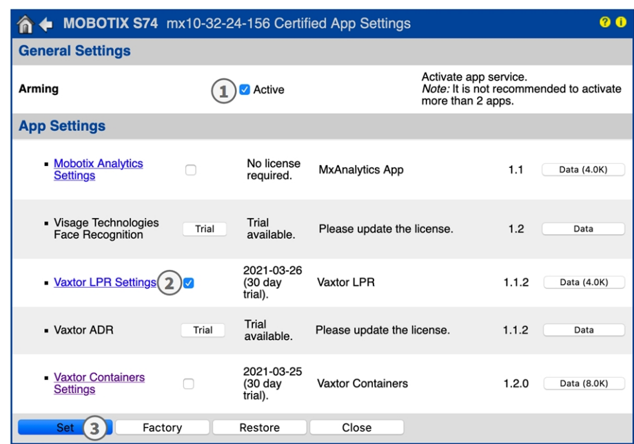
Fig. 11: Activation of Certified Apps
