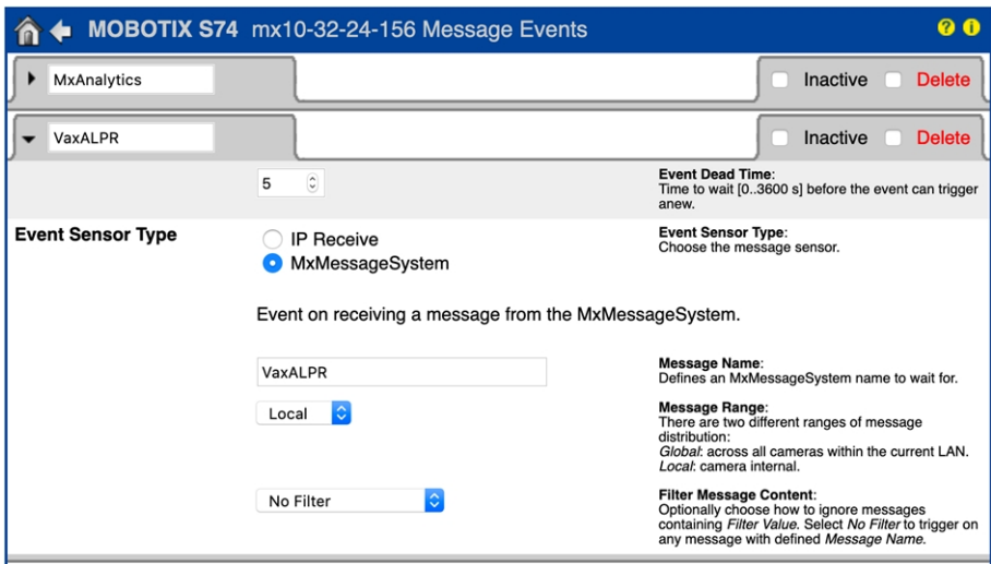
Fig. 23: Example: Generic message event details - no filter
