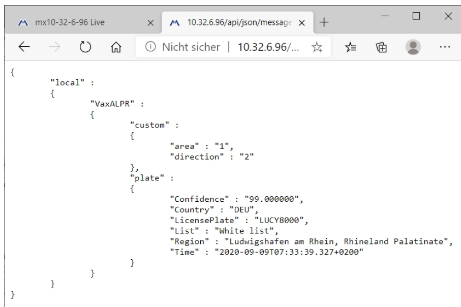
Fig. 28: Example: Meta data transmitted within an MxMessage of the VAXTOR License Plate Recognition App
