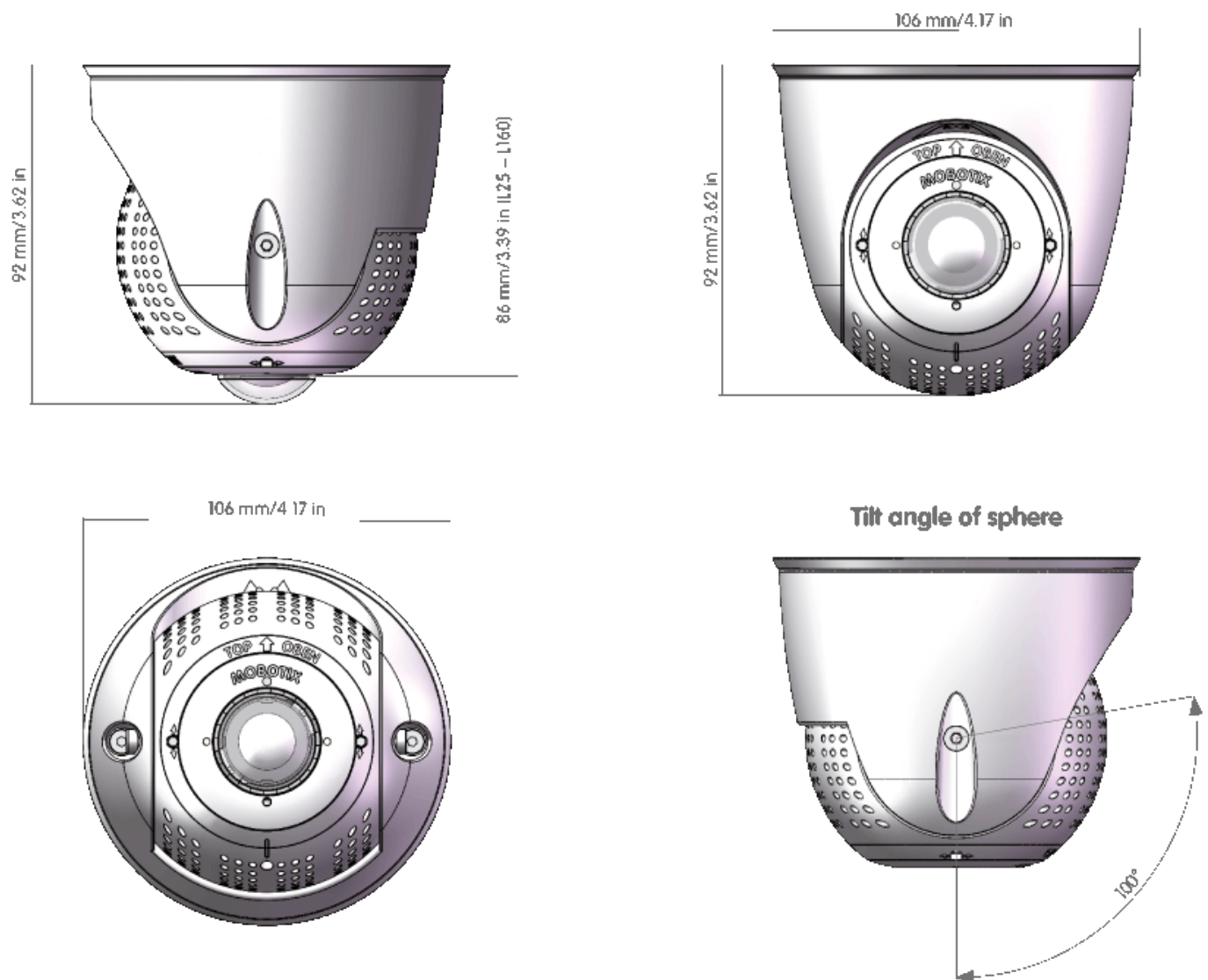
Fig. 6: PTMount
