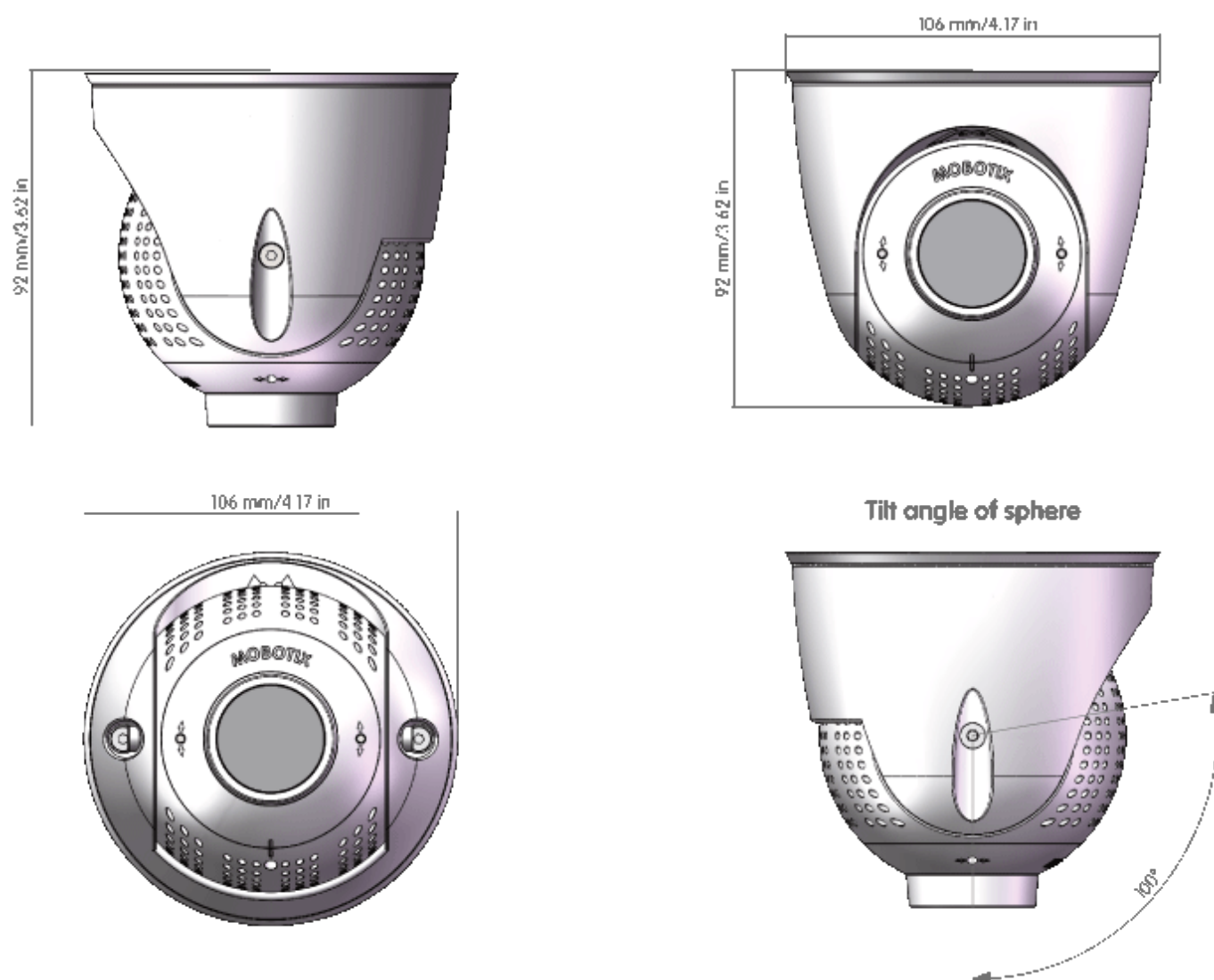
Fig. 7: PTMount-Thermal
