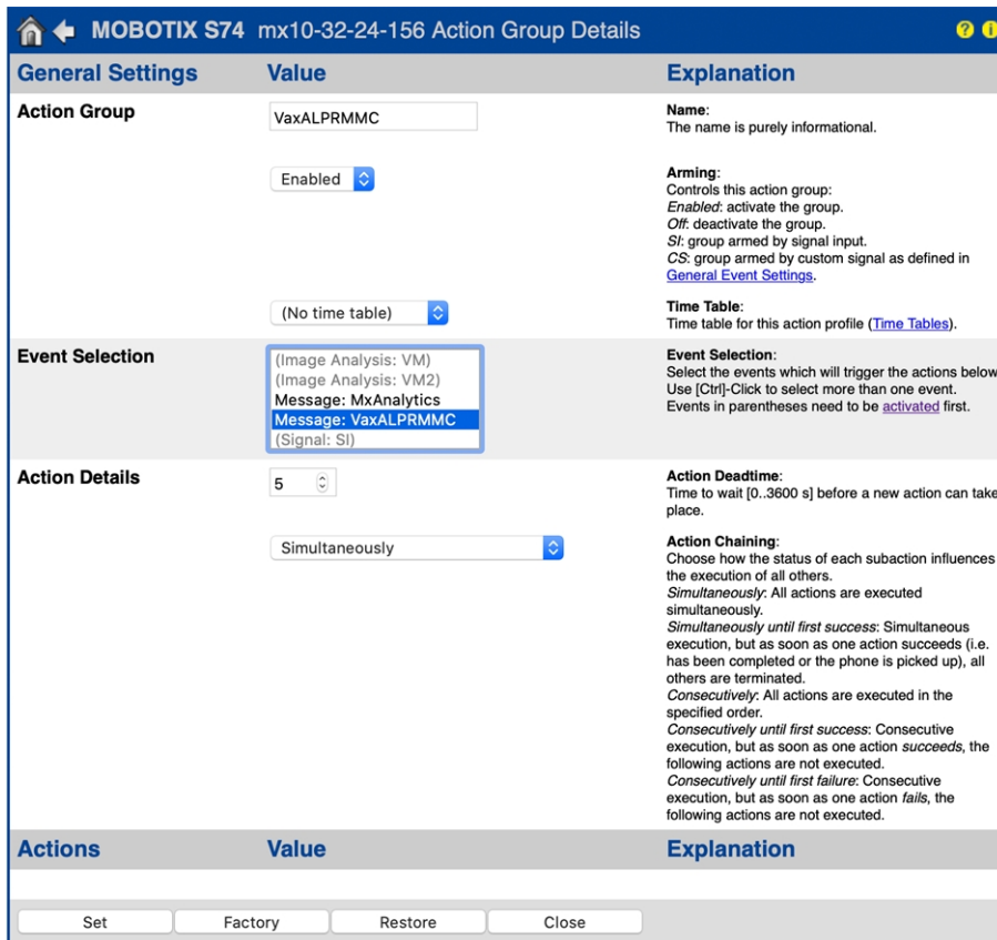
Fig. 24: Configuring an Action Group
