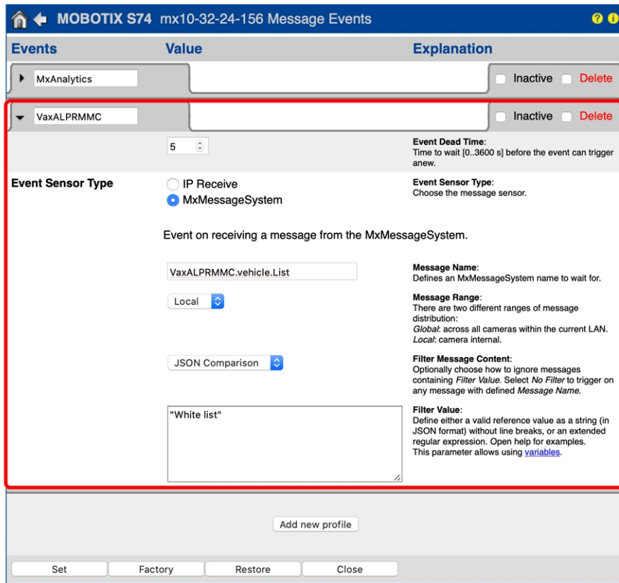
Fig. 28: Example: Configuration of a user-defined white list event
