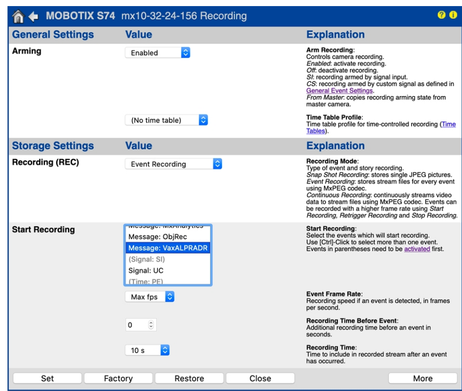
Fig. 26: Configuration of camera recording settings
