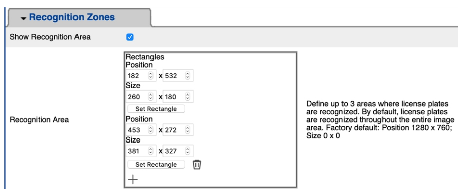
Fig. 20: Recognition Areas
