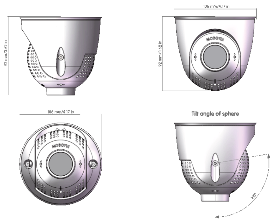
Fig. 7: PTMount-Thermal
