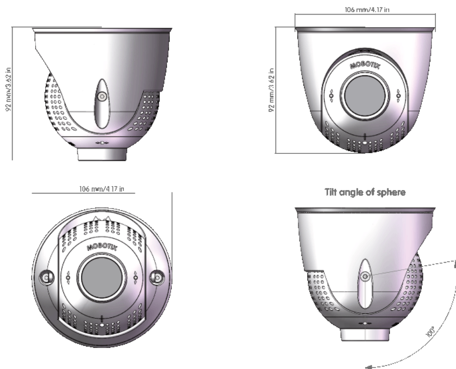
Fig. 7: PTMount-Thermal
