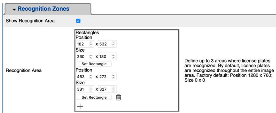
Fig. 22: Recognition Areas
