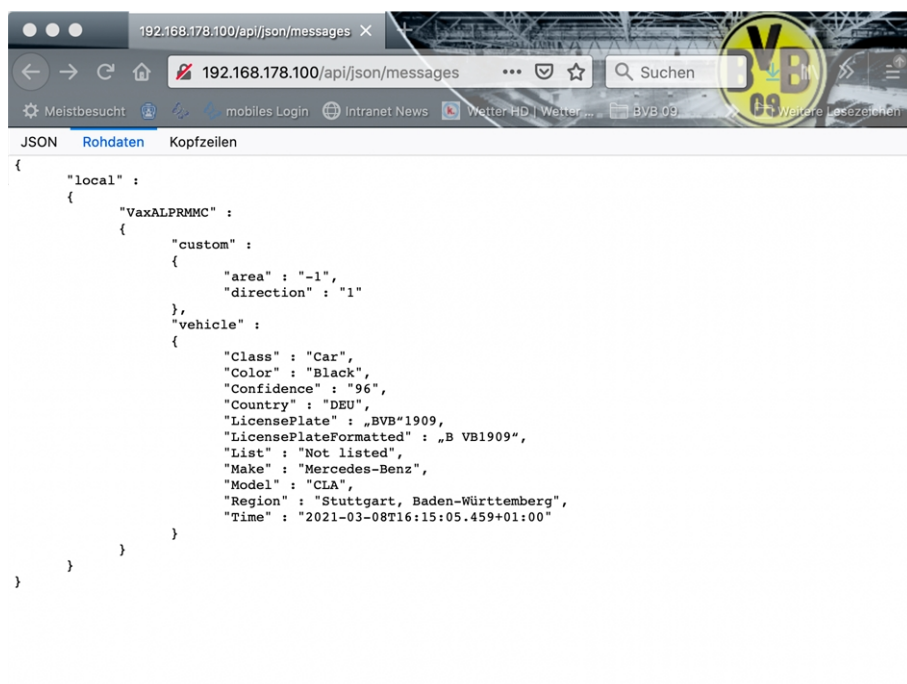
Fig. 28: Example: Meta data transmitted within an MxMessage of the Vaxtor LPR incl. Vehicle Make, Model, Color and Class App
