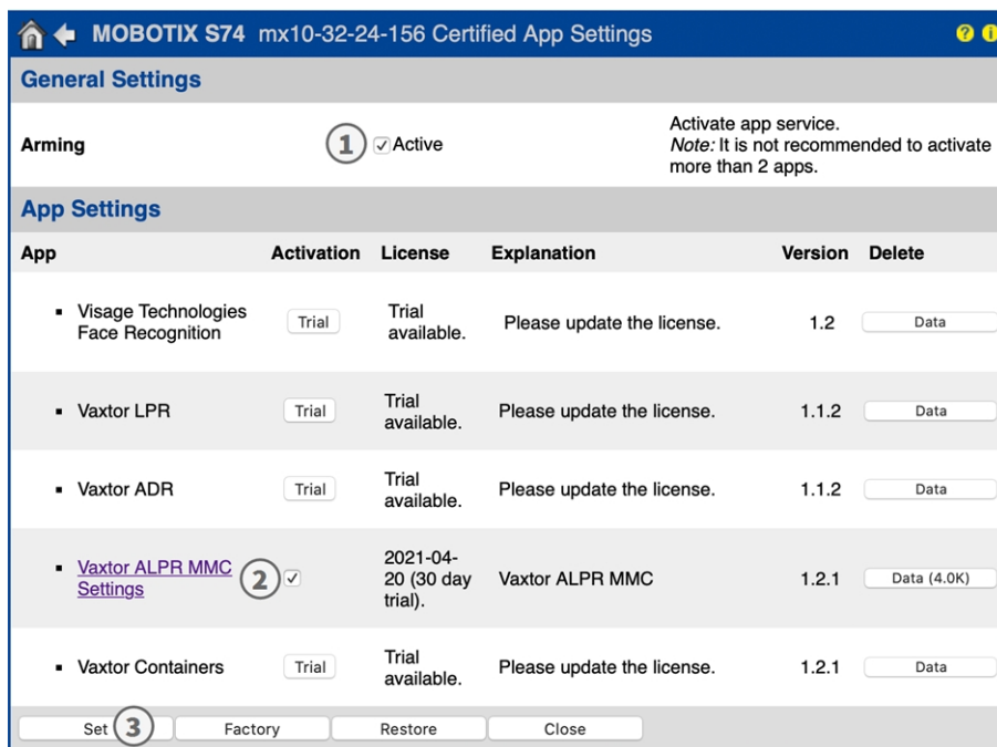
Fig. 12: Activation of Certified Apps
