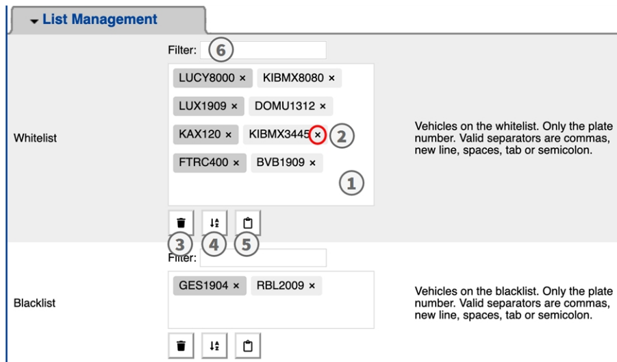
Fig. 15: Black and white lists
