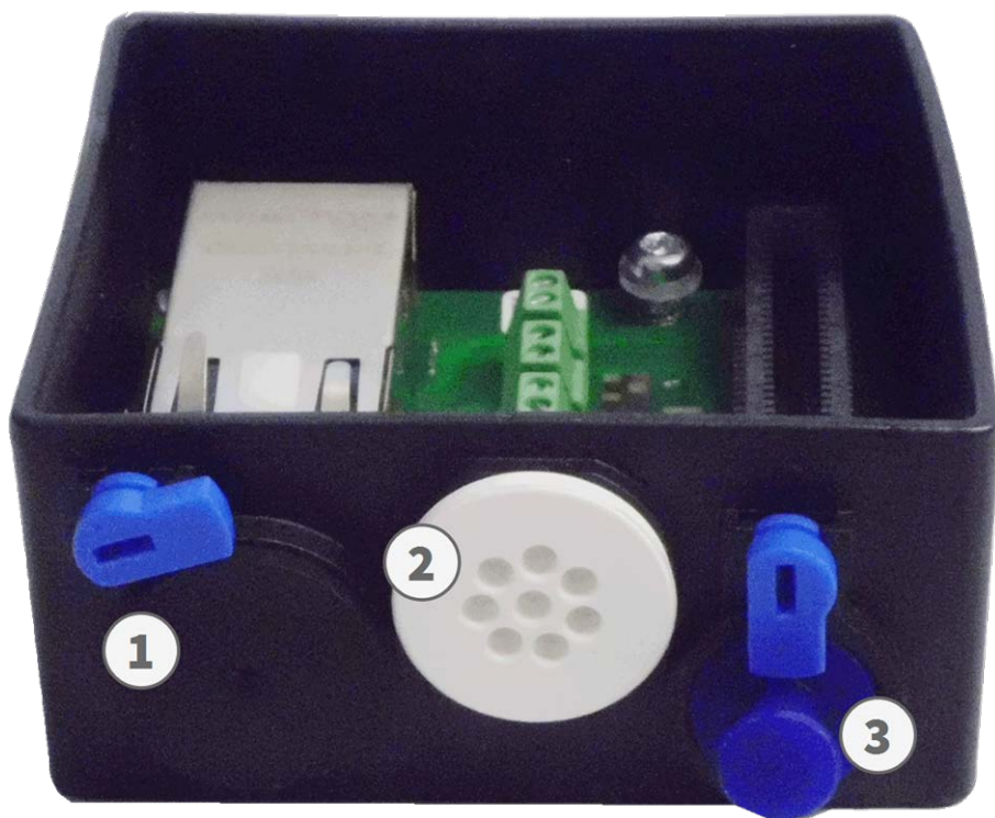
Fig. 32: Connector Box RJ45
