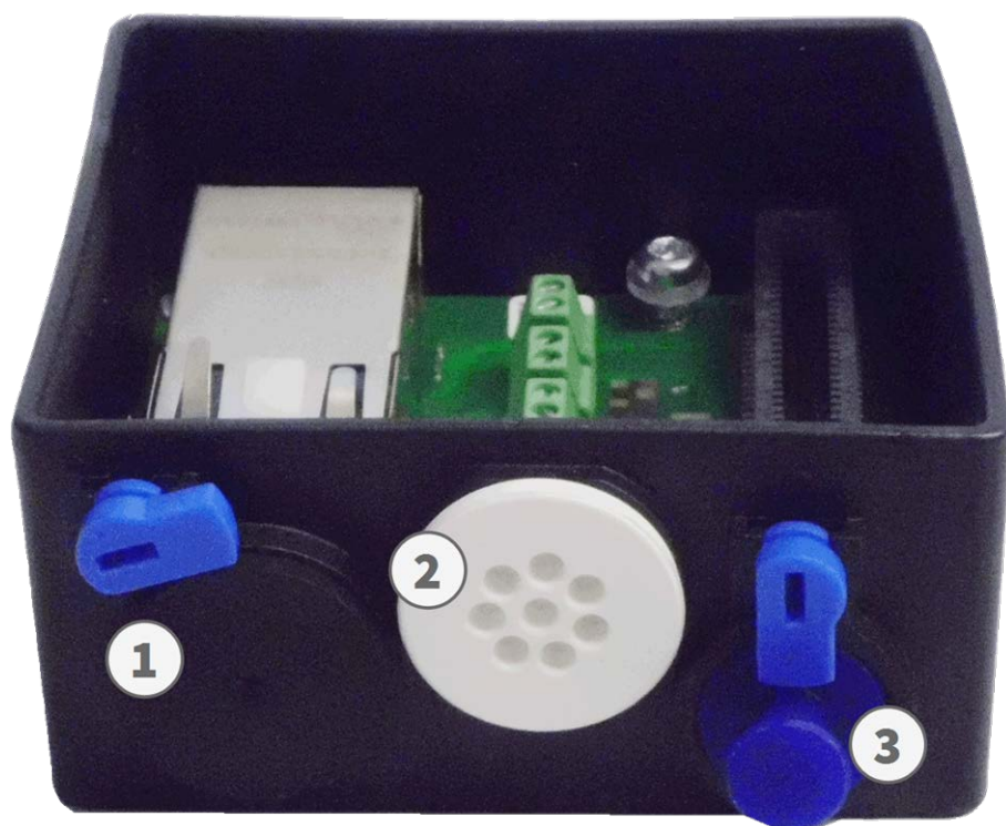
Fig. 47: Connector Box RJ45
