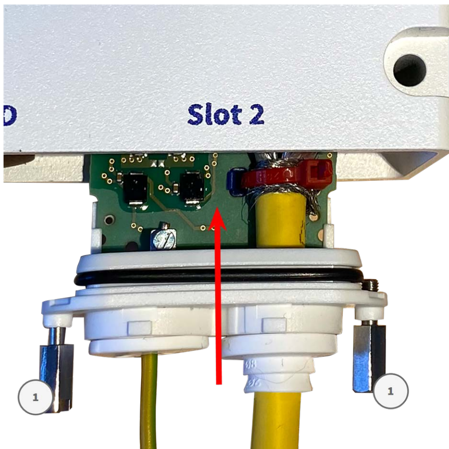
Fig. 30: Conexión del S74 network slide in board with LSA terminal
