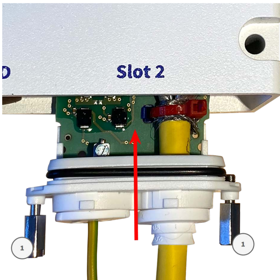
Fig. 30: Connexion du S74 network slide in board with LSA terminal
