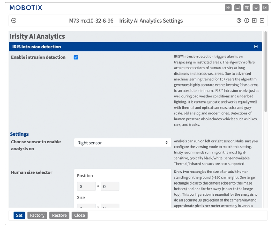
Fig. 14: Default operating mode: IRIS Intrusion detection
