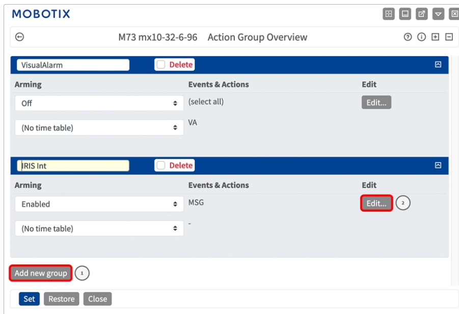
Fig. 21: Defining Action Groups
