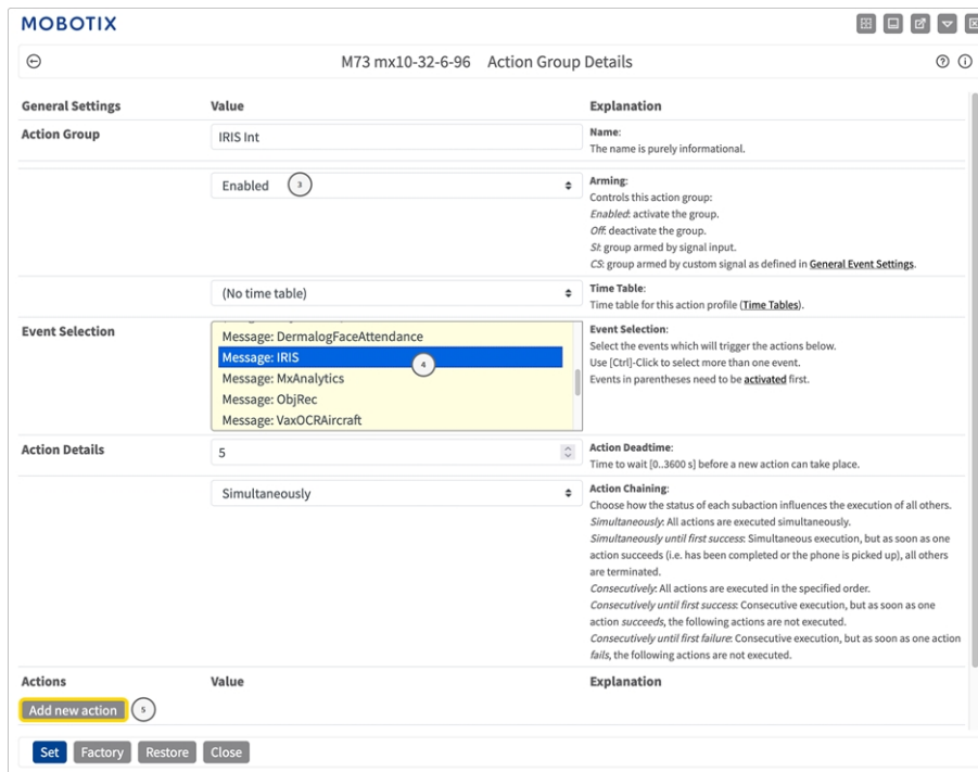
Fig. 22: Configuring an Action Group
