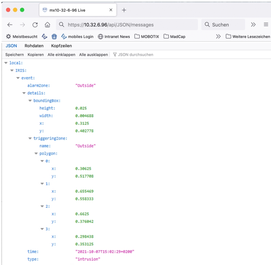
Fig. 25: Example: Meta data transmitted within an MxMessage of the Irisity IRIS Core AI Analytics - Intrusion Detection
