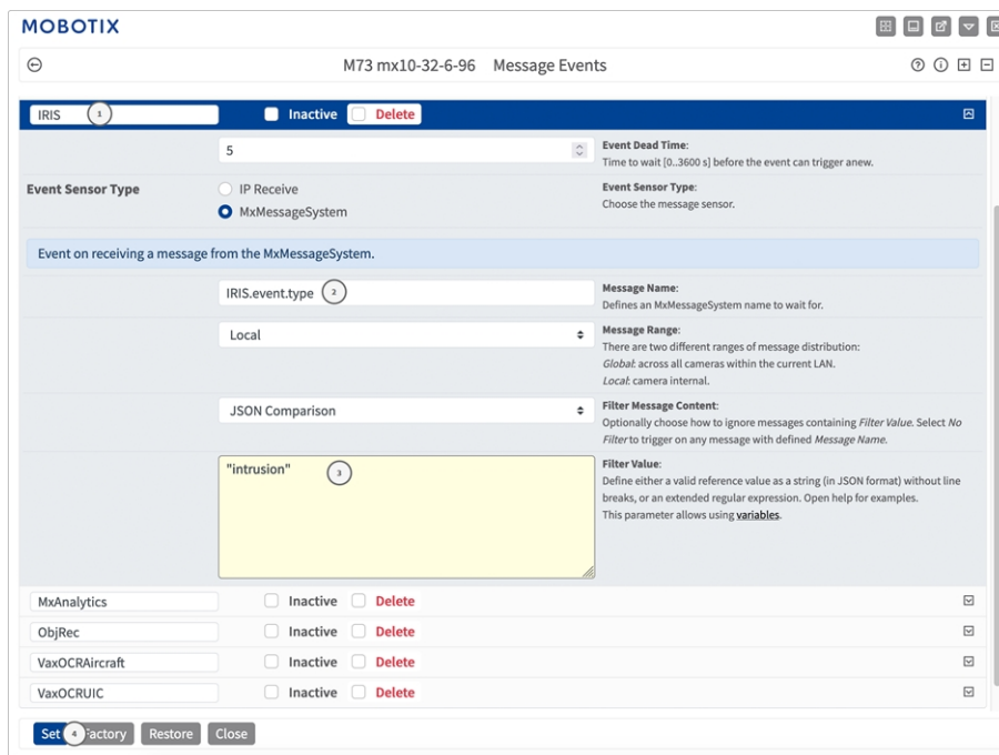
Fig. 27: Example: Intrusion message event
