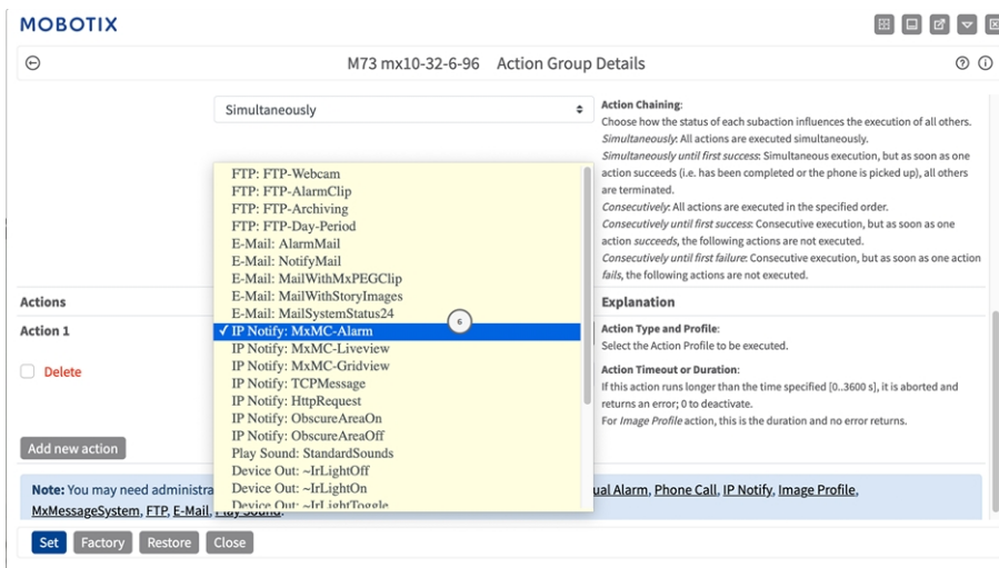
Fig. 23: Select Action Type- and Profile
