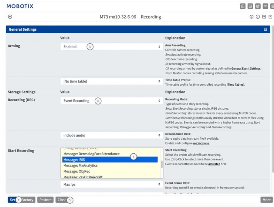
Fig. 24: Configuration of camera recording settings
