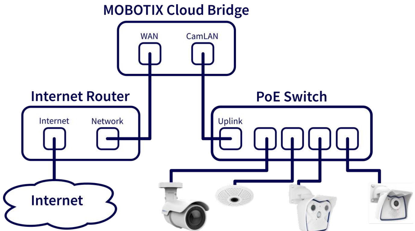
Fig. 1: Wiring diagram for the MOBOTIX Cloud Bridge
