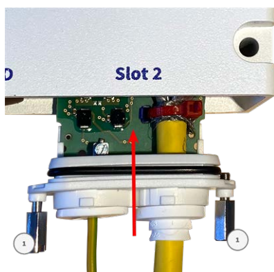
Fig. 30: Connecting the S74 Network slide in board with LSA terminal
