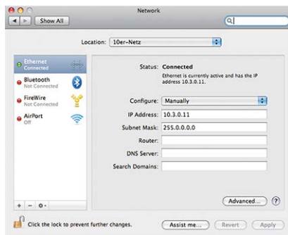
Fig. 39: Network settings on macOS machines
