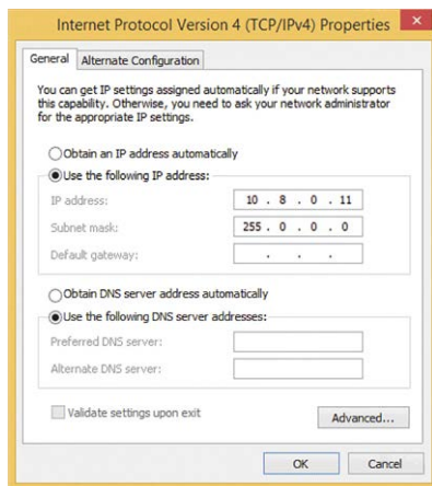
Fig. 38: Properties of Internet Protocol V4
