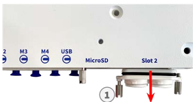
Fig. 22: Remove cover from interface board slot
