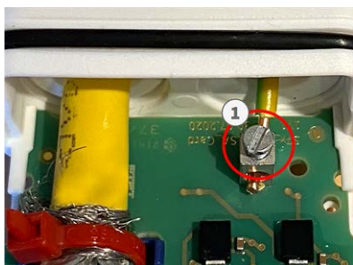
Fig. 29: Ground wire connected to terminal
