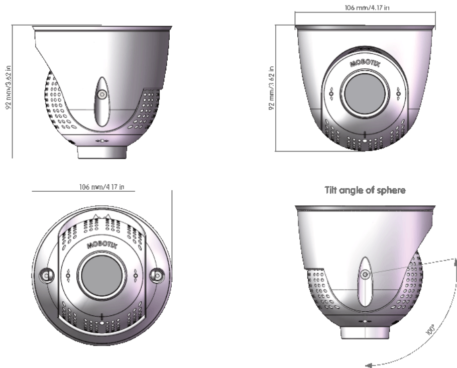
Fig. 7: PTMount-Thermal
