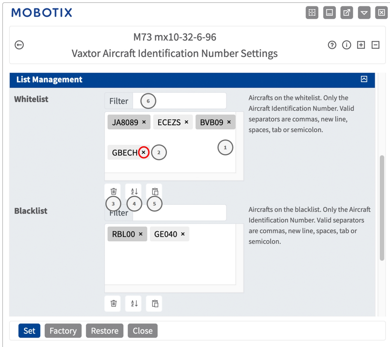
Fig. 15: Black and white lists
