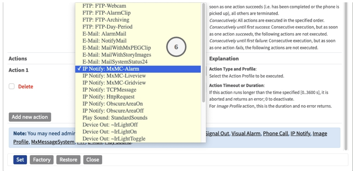
Fig. 27: Select Action Type- and Profile
