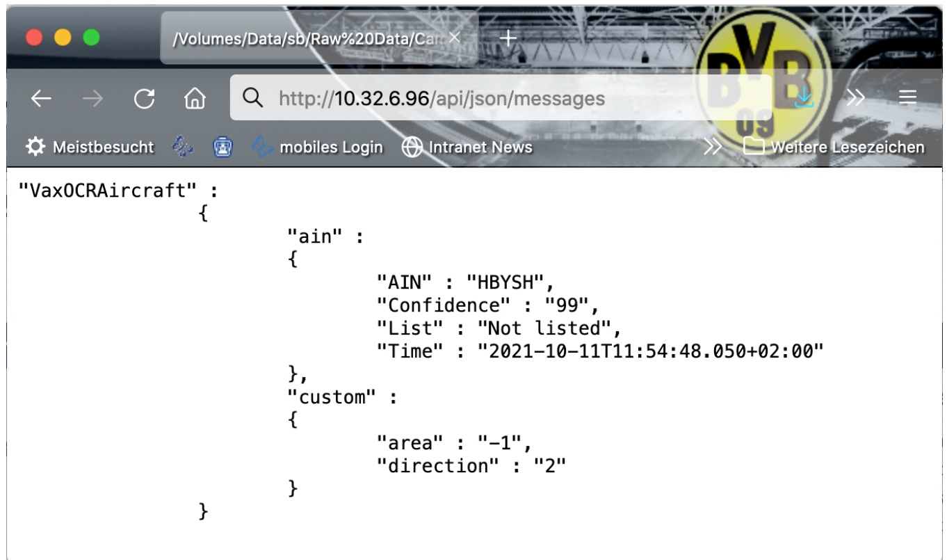
Fig. 30: Example: Meta data transmitted within an MxMessage of the Vaxtor Aircraft Identification Number Recognition App
