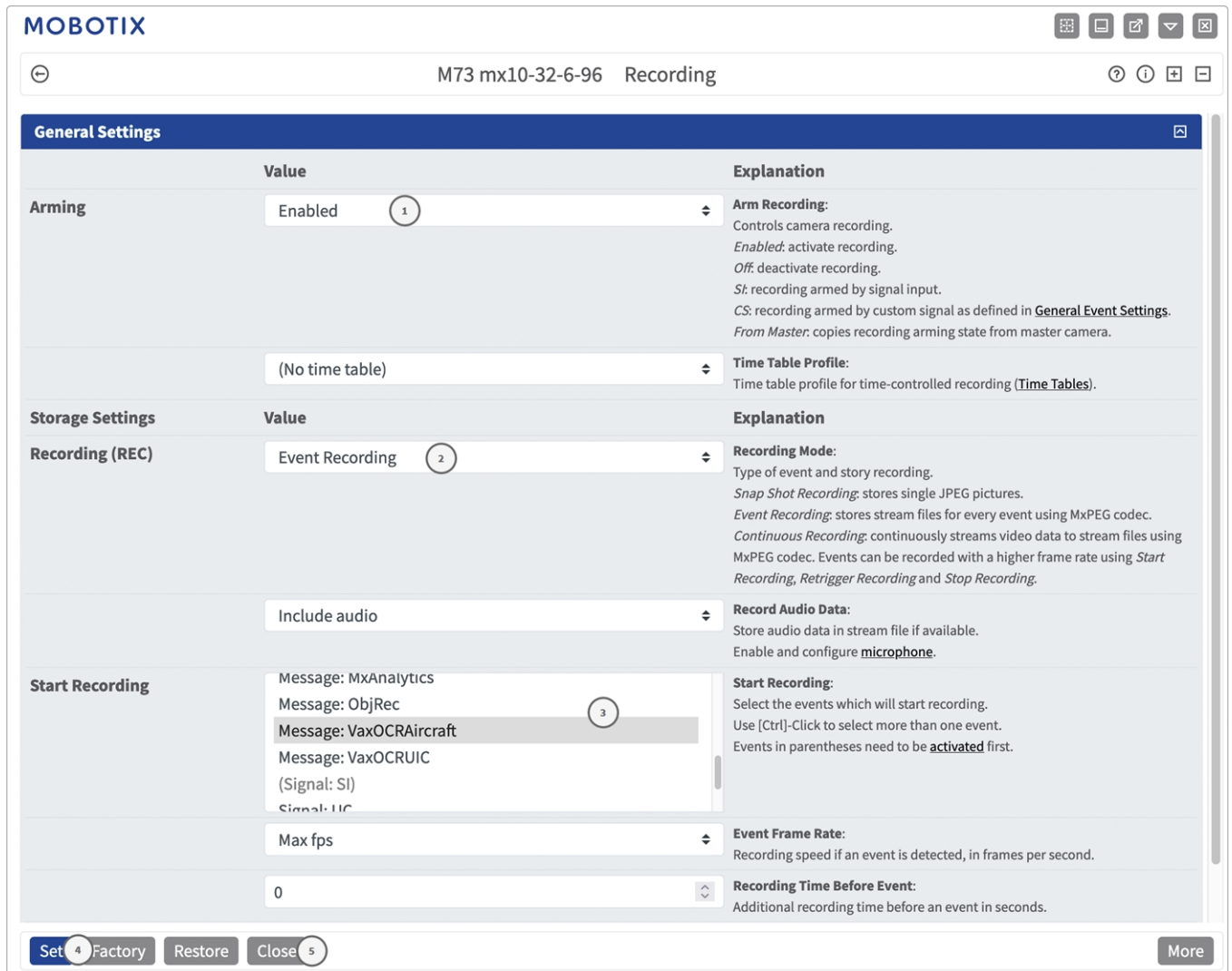
Fig. 28: Configuration of camera recording settings
