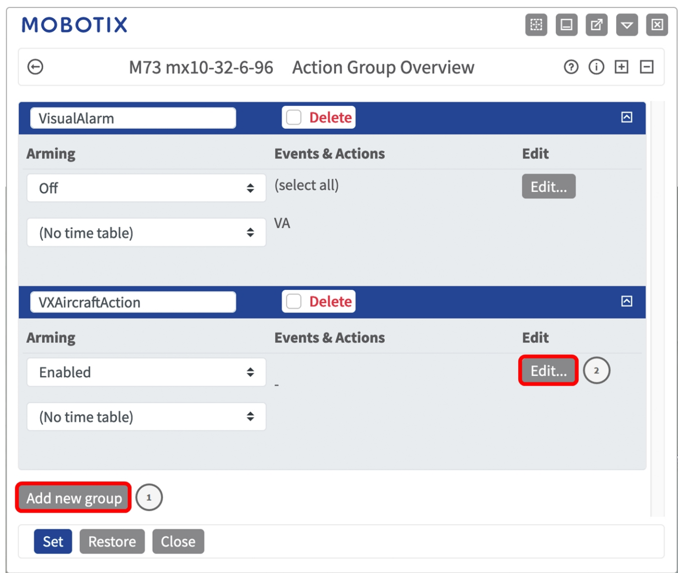
Fig. 25: Defining Action Groups
