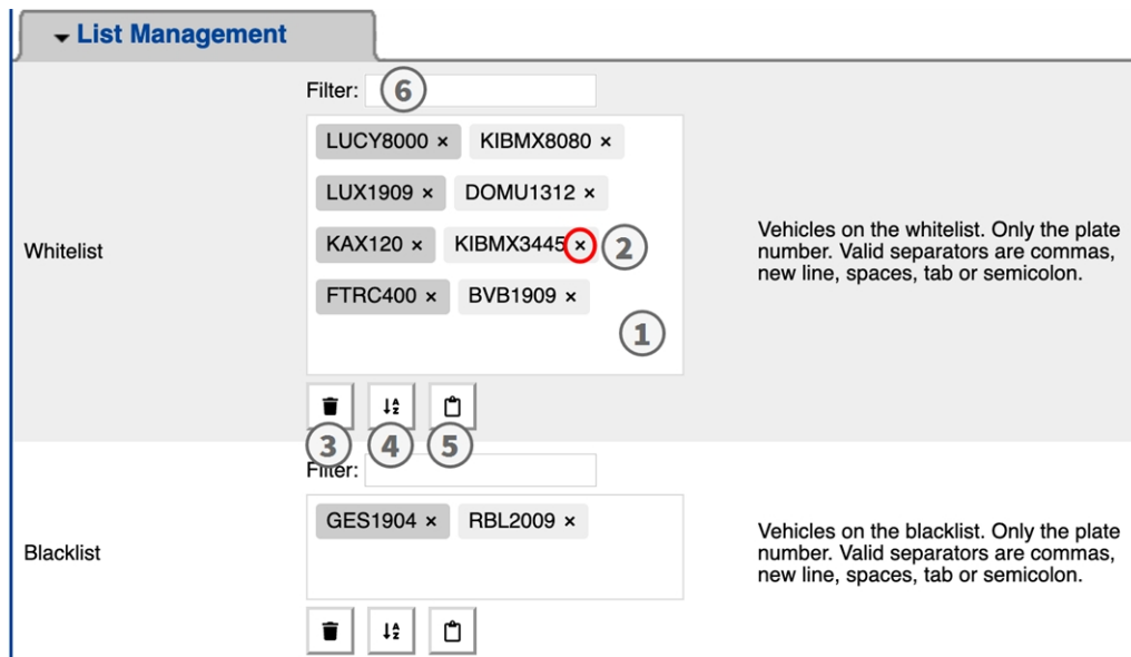
Fig. 15: Black and white lists
