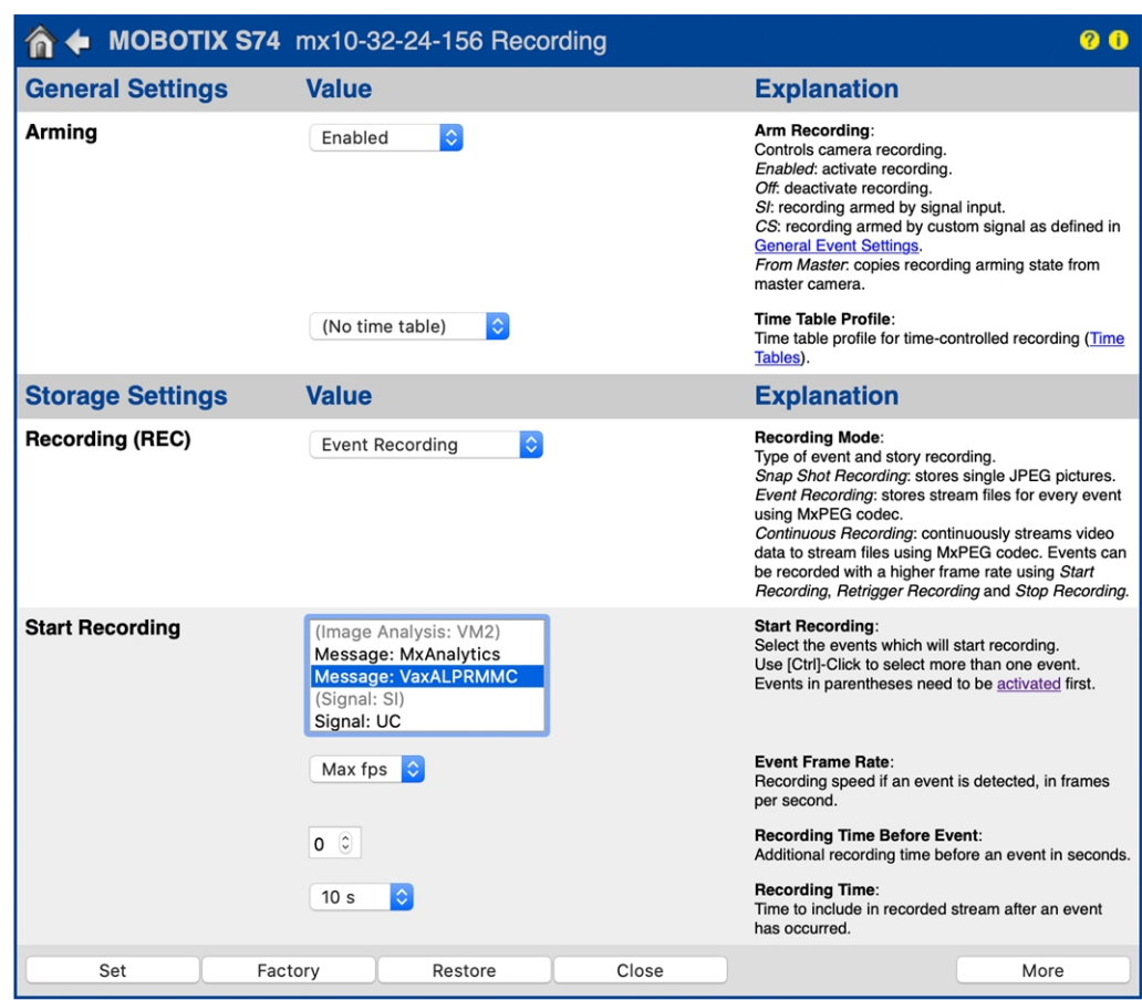
Fig. 27: Configuration of camera recording settings
