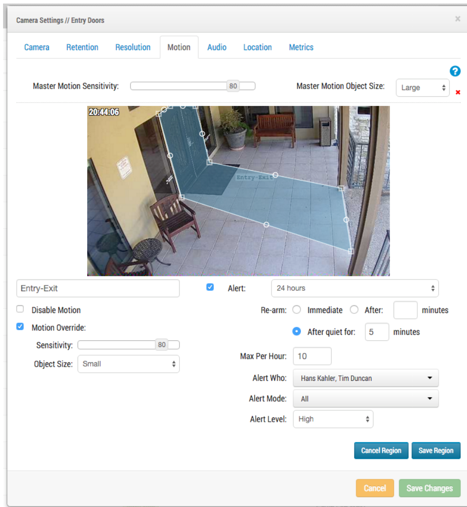
Fig. 65: Motion settings
