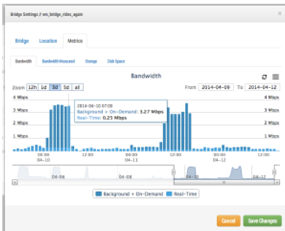
Fig. 80: Bandwidth metrics for bridge settings
