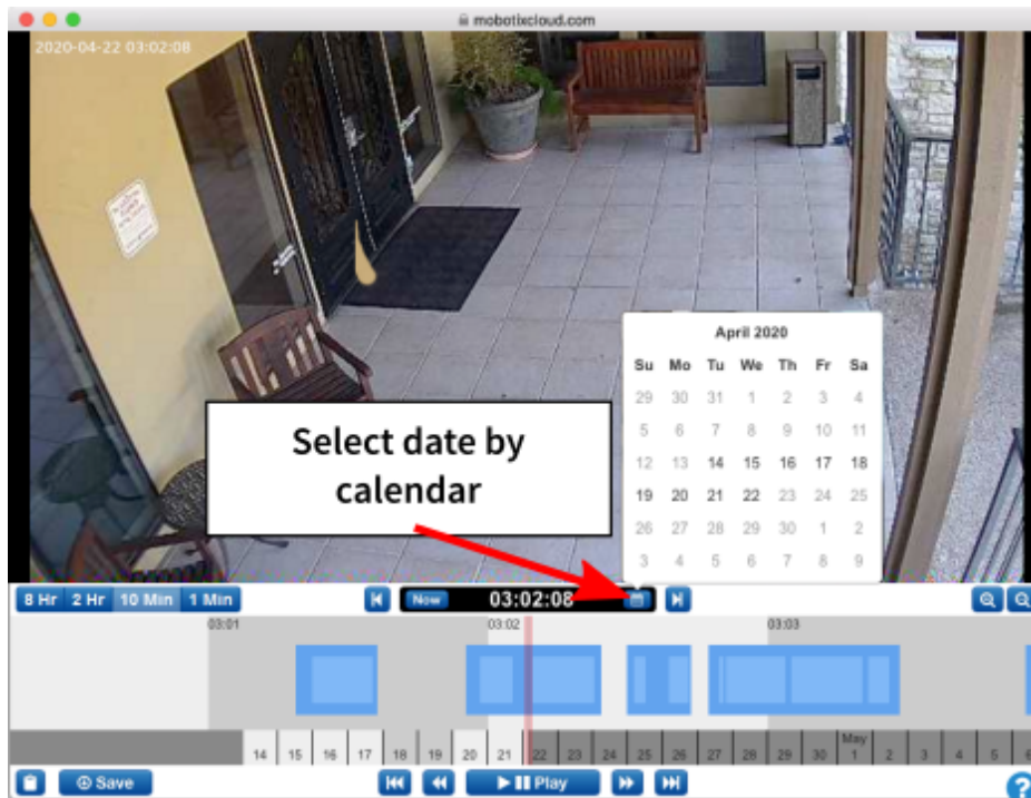
Fig. 48: History Browser calendar
