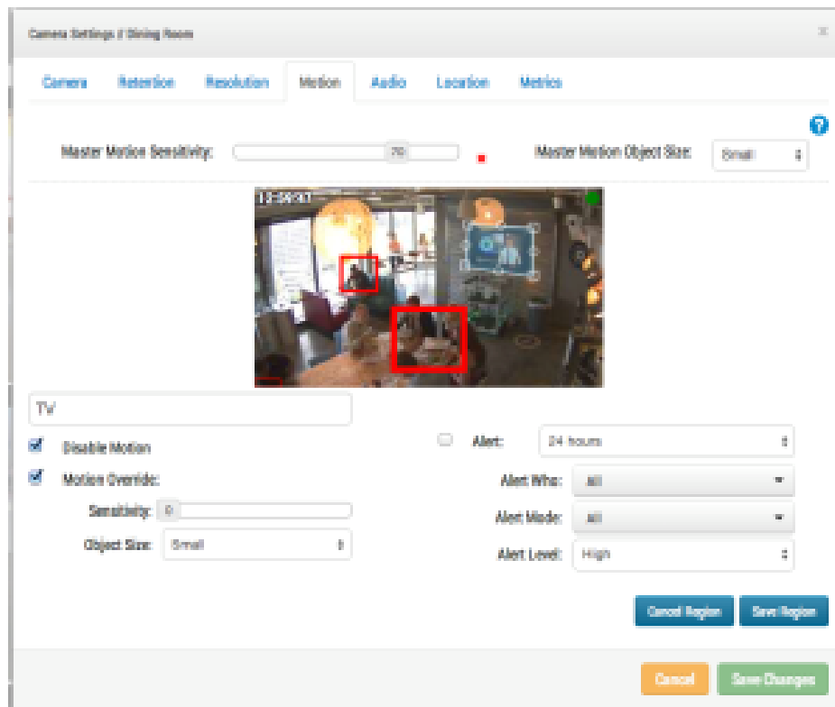
Fig. 61: Motion detection exclusion zone settings
