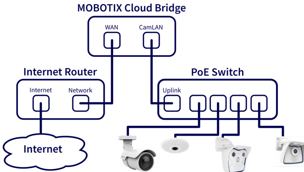
Fig. 1: Wiring diagram for the MOBOTIX Cloud Bridge
