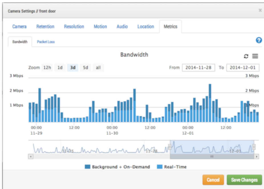
Fig. 22: Camera bandwidth utilization
