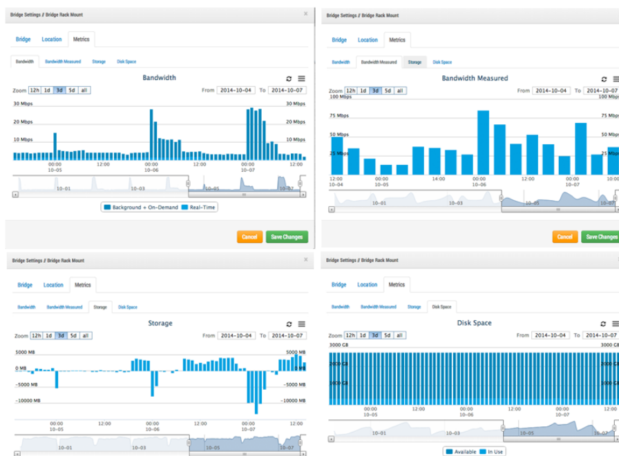
Fig. 71: Bandwidth example 1
