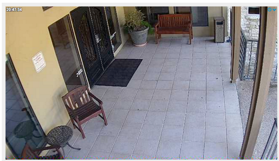
Fig. 64: Camera view
