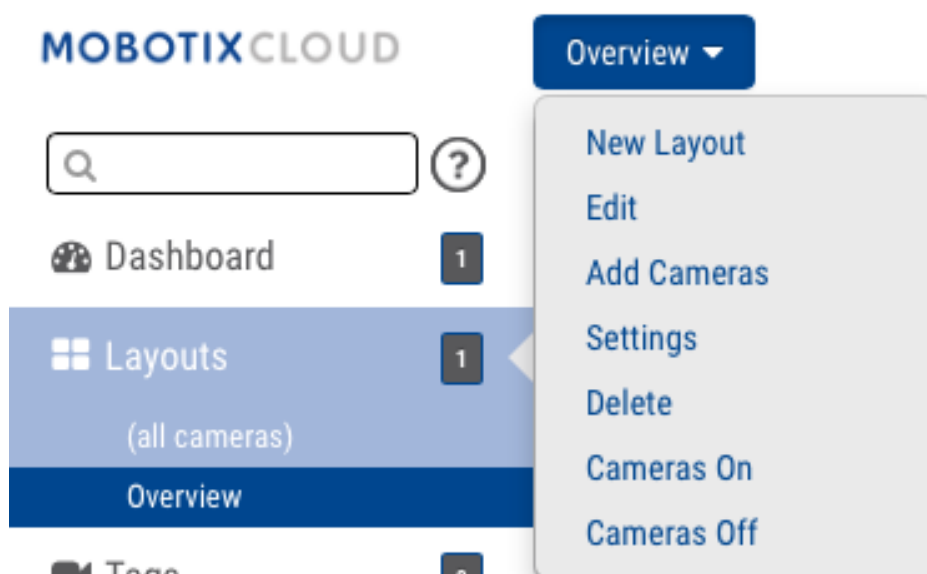
Fig. 13: Layouts menu
