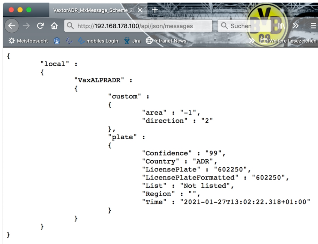
Fig. 27: Example: Meta data transmitted within an MxMessage of the Vaxtor License Plate Recognition / Dangerous Goods App
