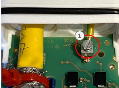
Fig. 28: Ground wire connected to terminal
