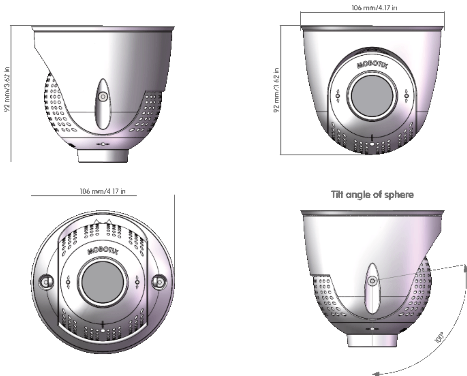
Fig. 7: PTMount-Thermal
