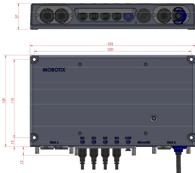
Fig. 5: S74: All measurements in mm
