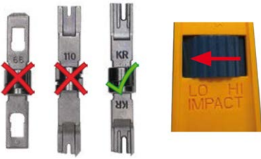
Fig. 25: LSA+/Krone tool set to LOW impact
