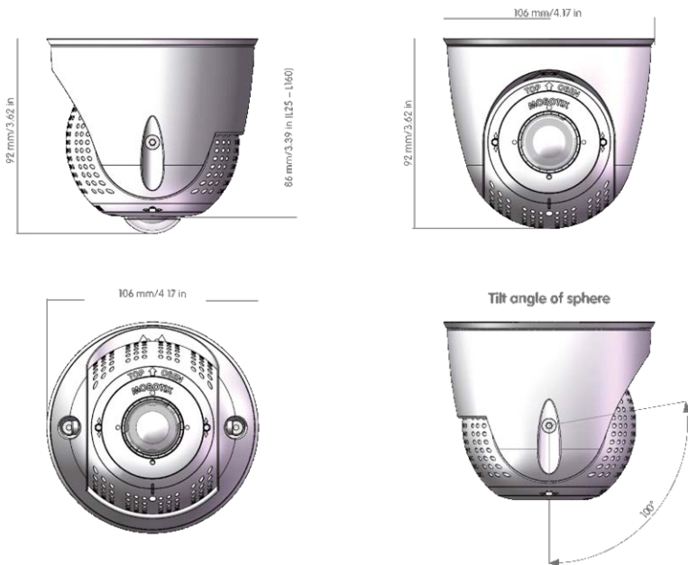
Fig. 6: PTMount
