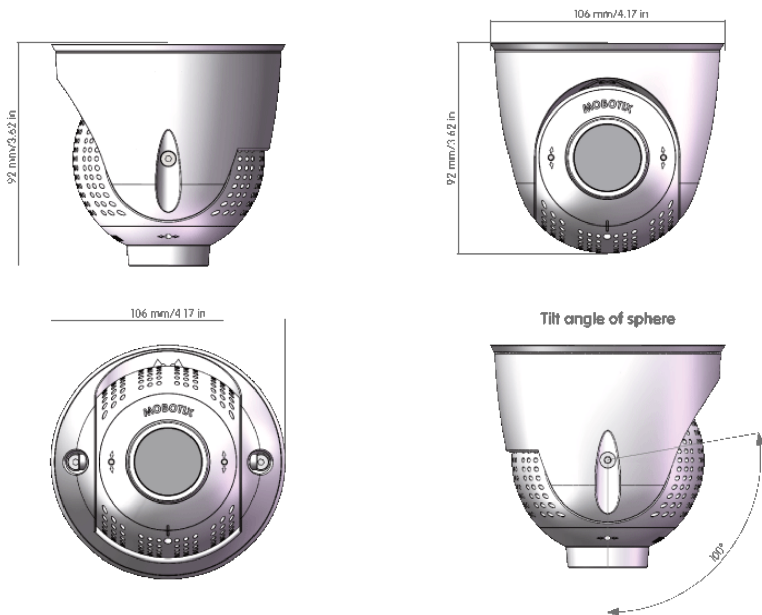
Fig. 7: PTMount-Thermal
