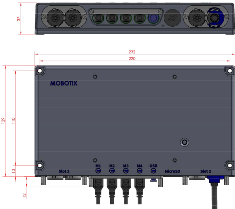
Fig. 5: MOBOTIX S74: All measurements in mm
