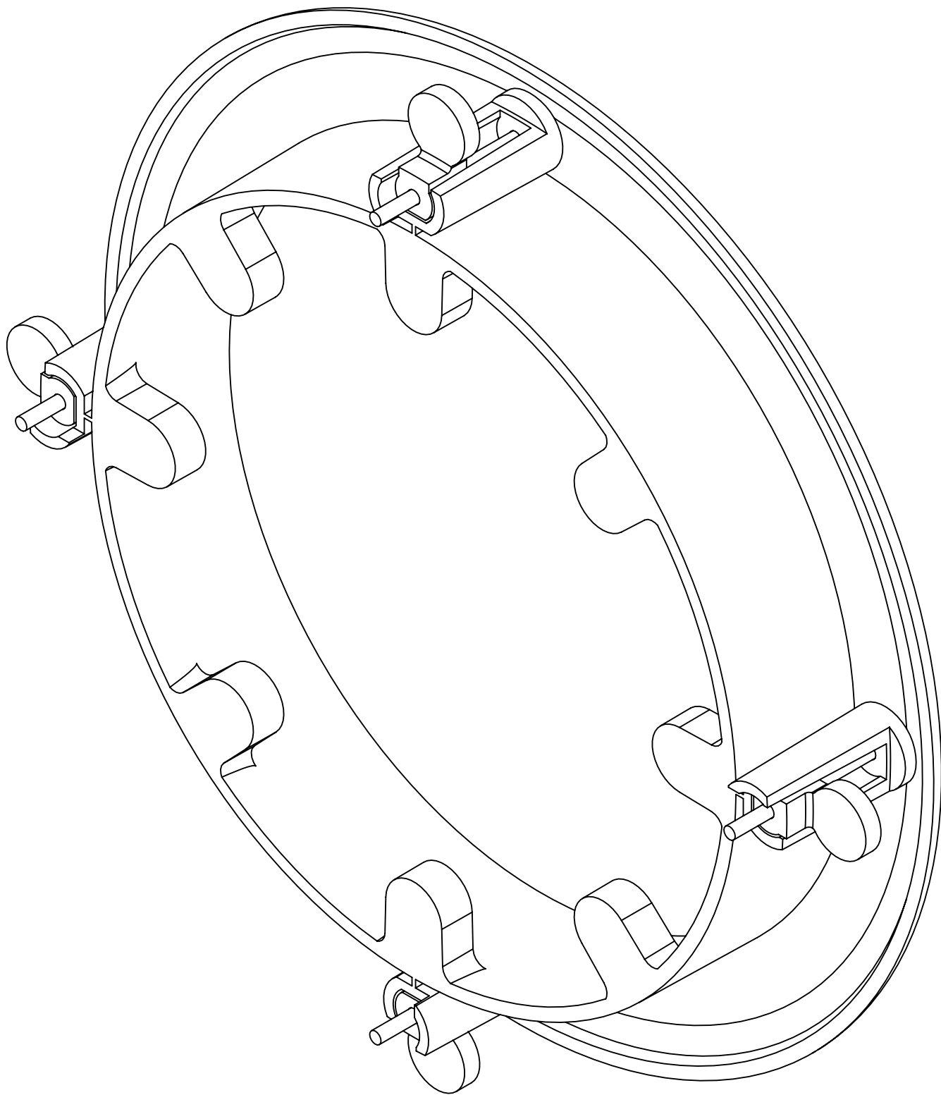
Isometric view
