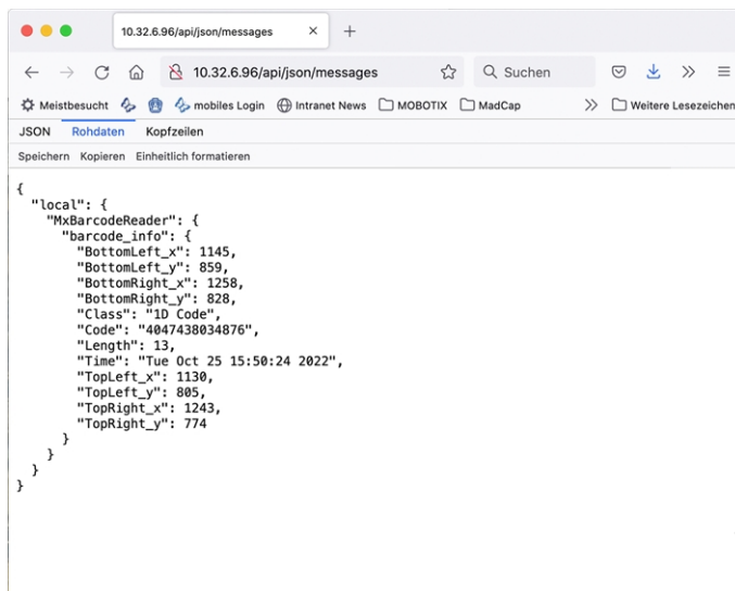
Fig. 22: Example: Meta data transmitted within a MxMessage of the MOBOTIX Barcode Reader App
