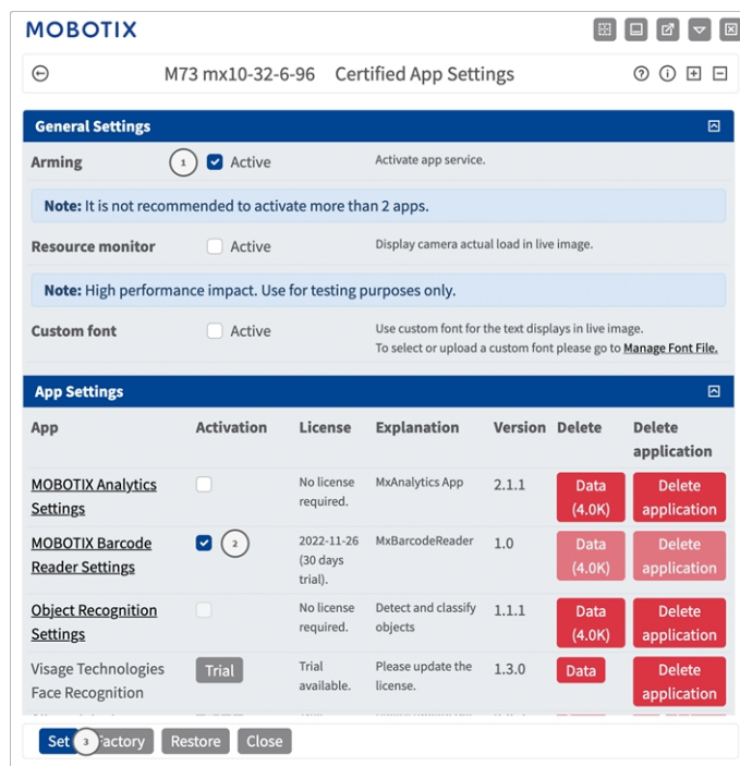
Fig. 10: Certified App: Settings
