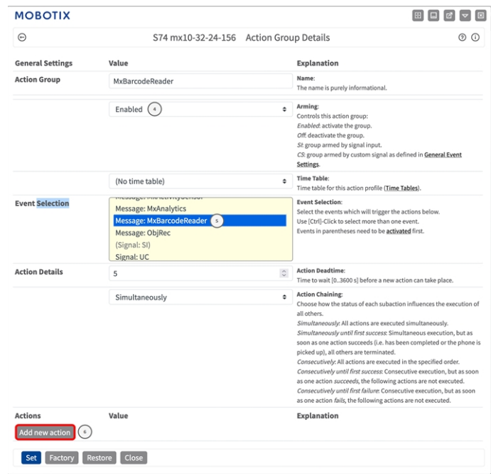
Fig. 19: Configuring an Action Group
