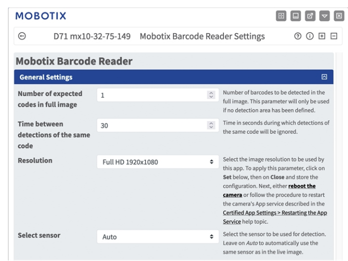
Fig. 11: General Settings
