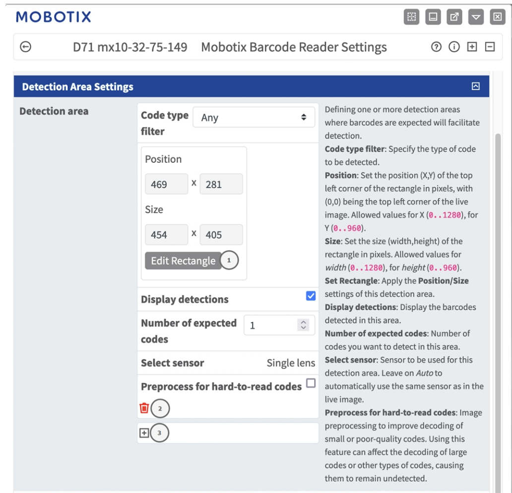
Fig. 13: Detection settings
