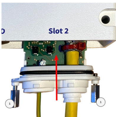
Fig. 29: Conexión del S74 Network Slide in Board with LSA terminal
