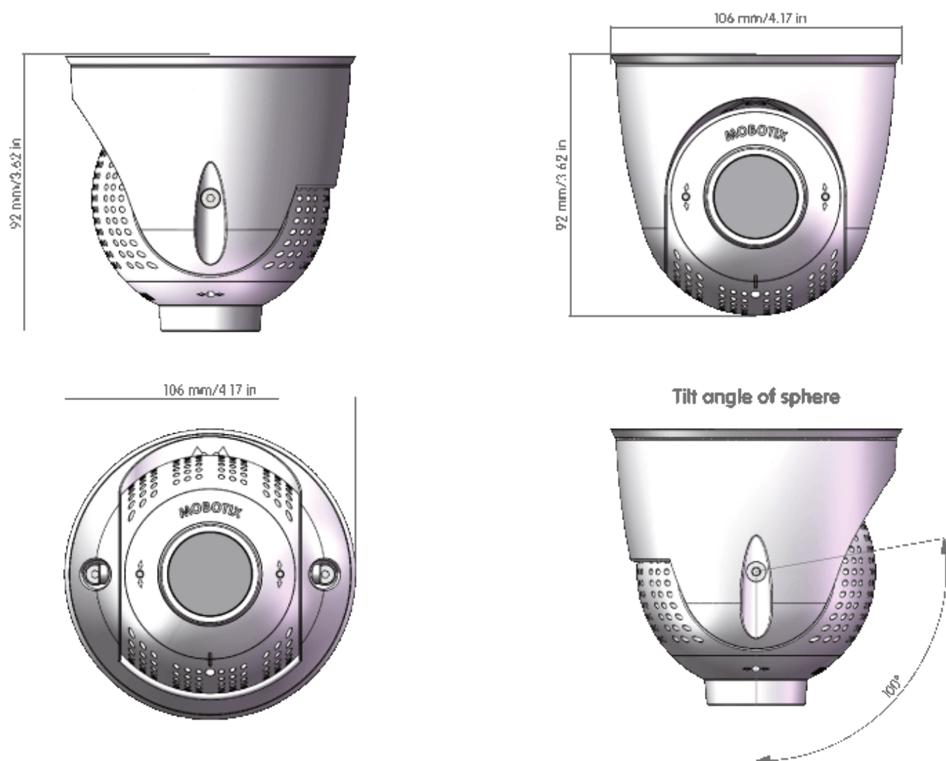
Fig. 7: PTMount-Thermal
