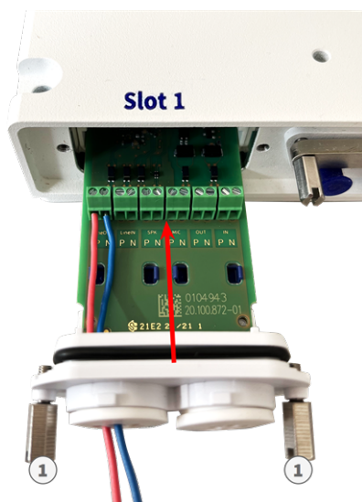
Fig. 34: Conexión del S74 Network Slide in Board with RJ45 socket
