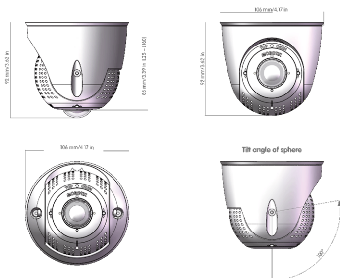
Fig. 6: PTMount
