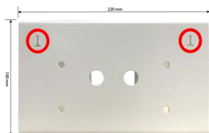
Fig. 10: Dimensiones MOBOTIX p71 Corner/Pole Mount: vista frontal
