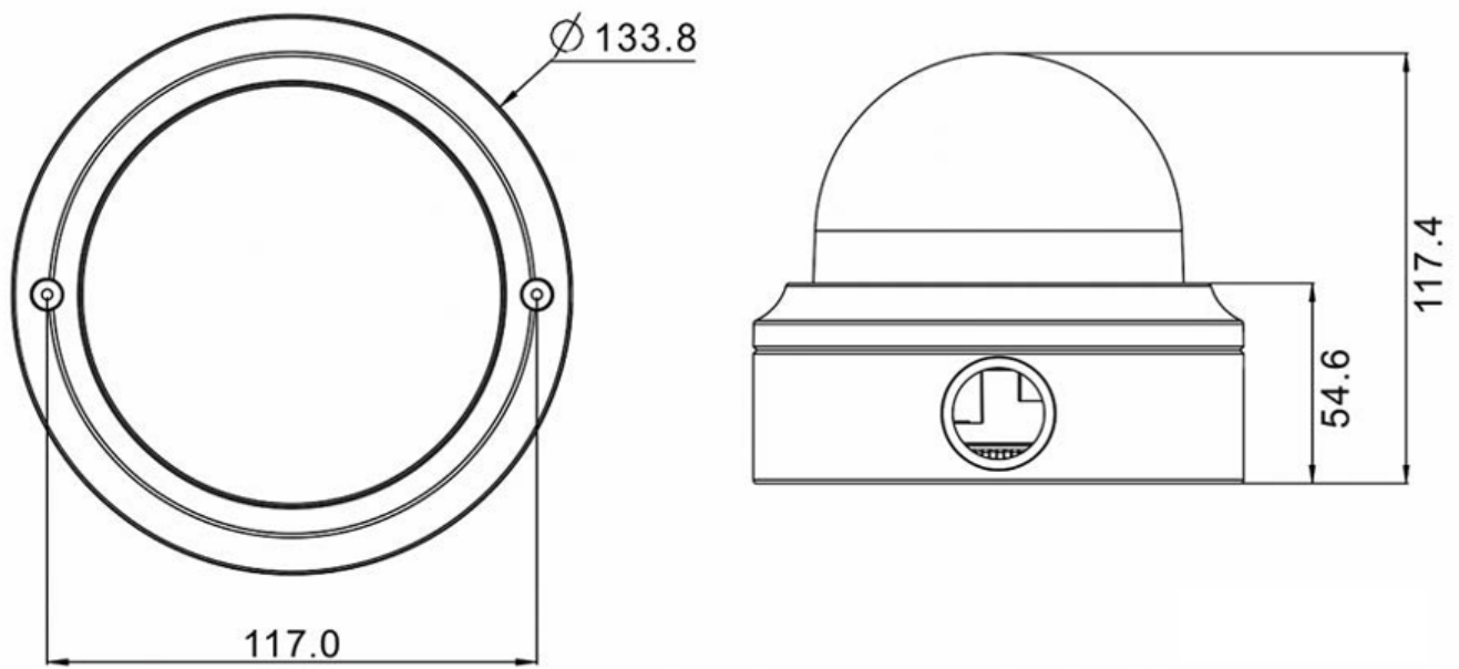
Fig. 1: 5MP Vandal Fixed Dome Analytics Camera: All measurements in mm
