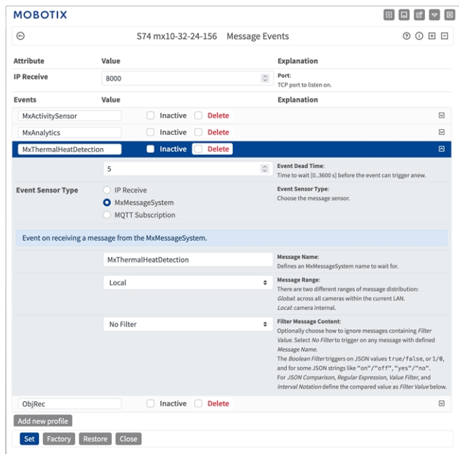
Fig. 23: Example: Generic message event details - no filter
