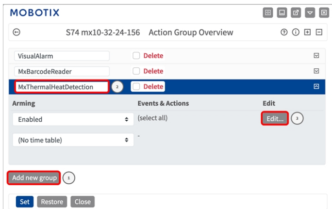
Fig. 24: Defining Action Groups
