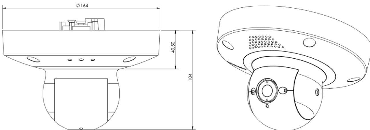
Fig. 1: MOBOTIX p71 ECO Thermal: All measurements in mm
