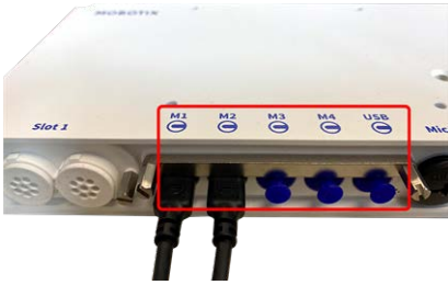
Fig. 37: 4 Module Connector Ports and 1 USB-C interface
