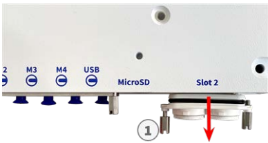
Fig. 21: Remove cover from interface board slot
