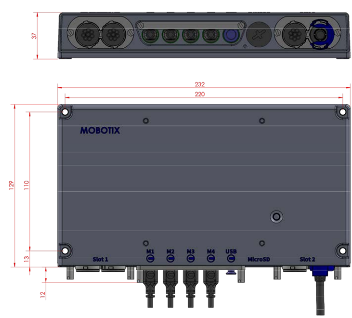
Fig. 5: MOBOTIX S74: All measurements in mm
