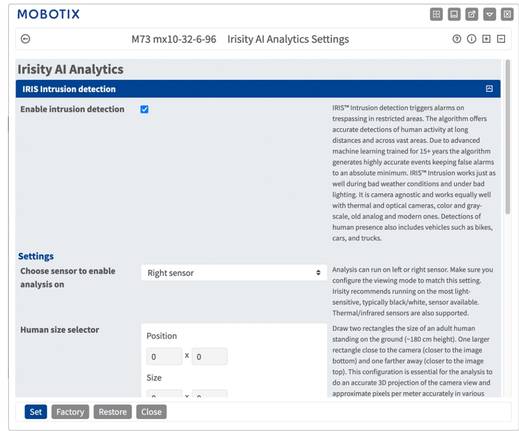
Fig. 14: Default operating mode: IRIS Intrusion detection
