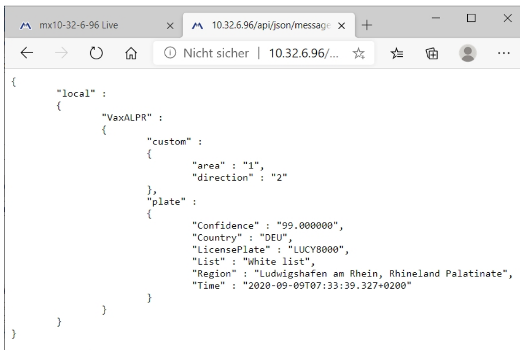
Fig. 29: Example: Meta data transmitted within a MxMessage of the Vaxtor License Plate Recognition App
