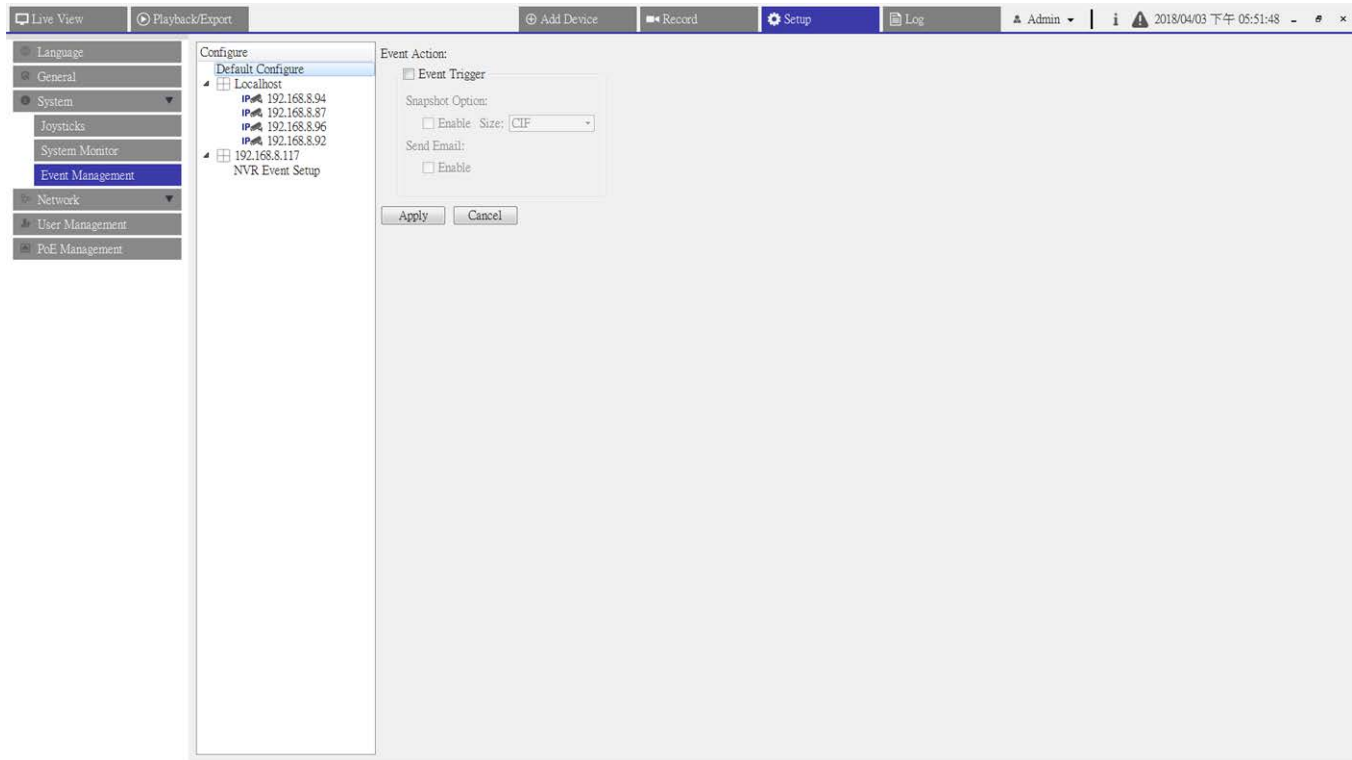
Fig. 19: Event setup
