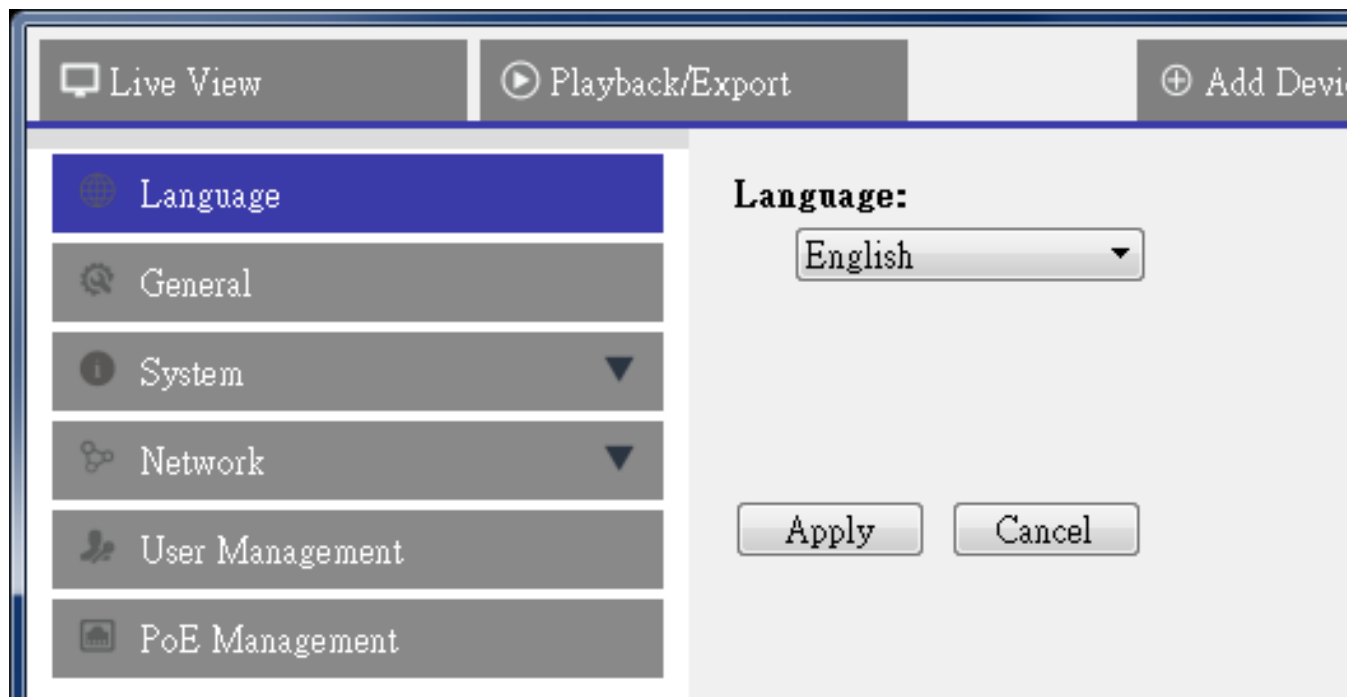
Fig. 15: Language setup
