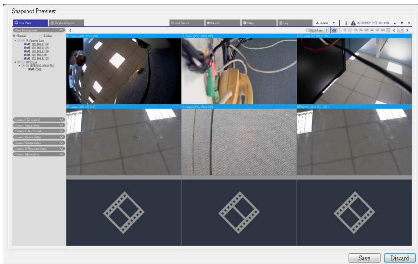
Fig. 7: Snapshot Preview
