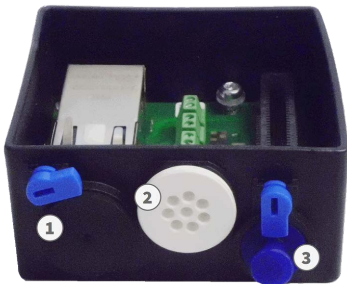
Abb. 46: Connector Box RJ45
