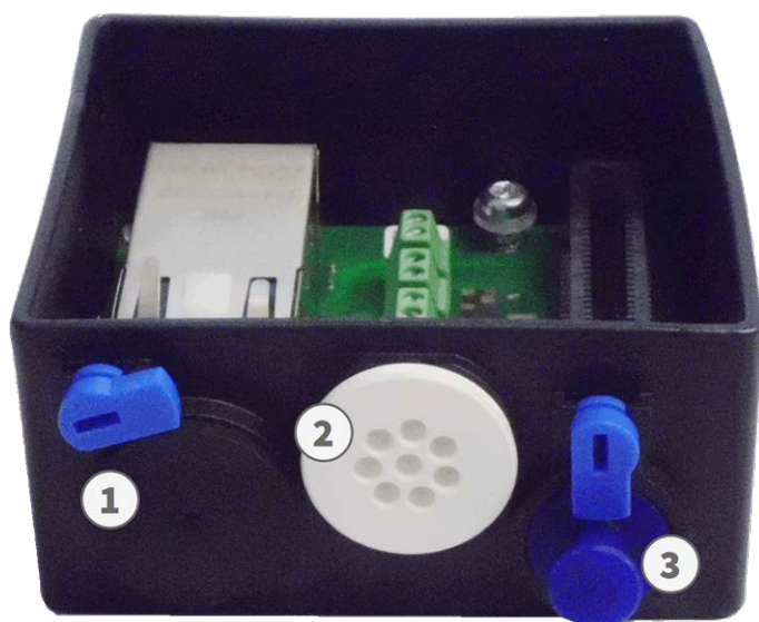
Abb. 32: Connector Box RJ45
