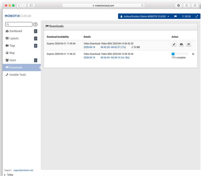
Fig. 41: Page Notifications
