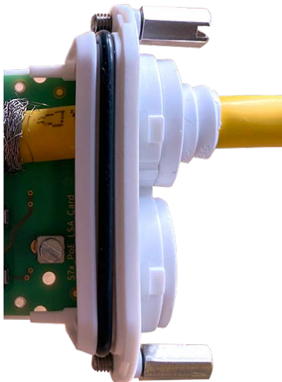
Fig. 13: Network cable inserted, plug properly seated
