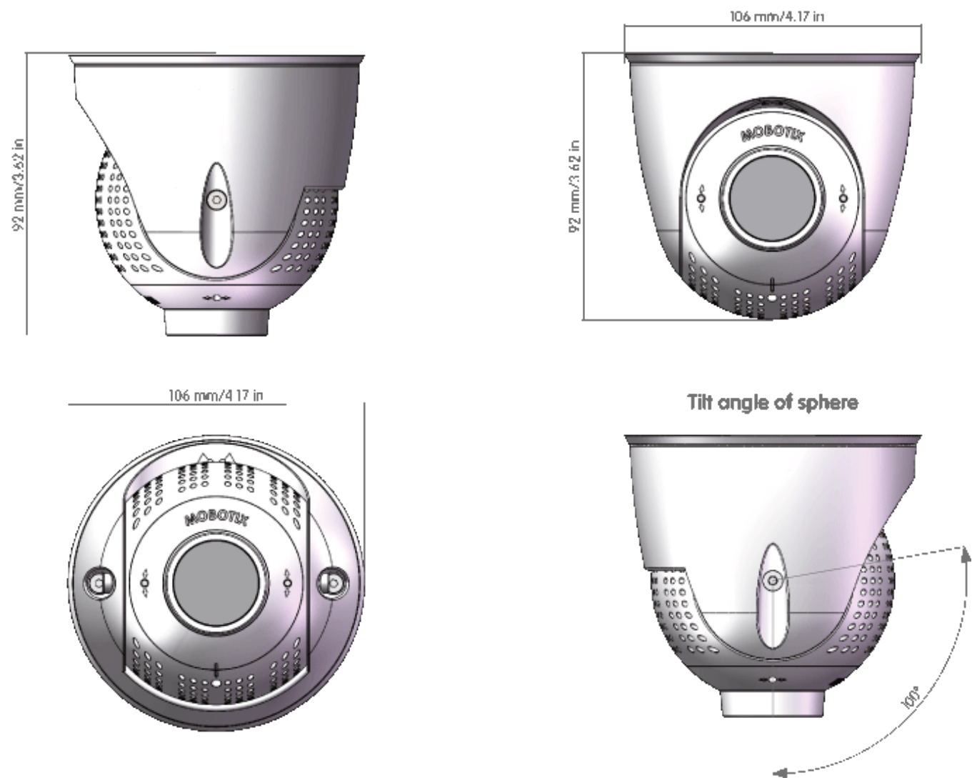
Fig. 6: PTMount-Thermal
