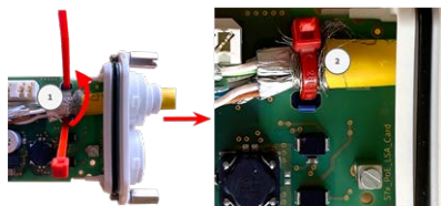
Fig. 14: Cable tie inserted beneath network cable
