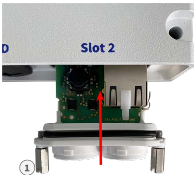
Fig. 9: Connecting the S74 Network Slide in Board with RJ45 socket
