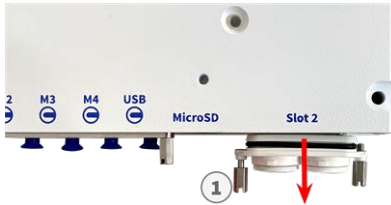
Fig. 8: Remove cover from interface board slot
