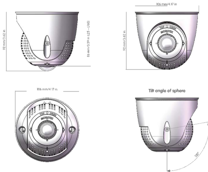
Fig. 5: PTMount
