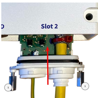
Fig. 19: Connecting the S74 Network Slide in Board with LSA terminal
