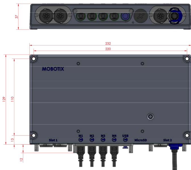
Fig. 4: MOBOTIX S74: All measurements in mm
