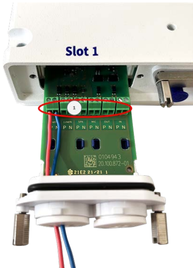
Fig. 22: IO wires connected to terminal
