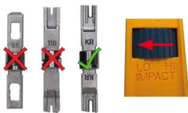
Fig. 15: LSA+/Krone tool set to LOW impact
