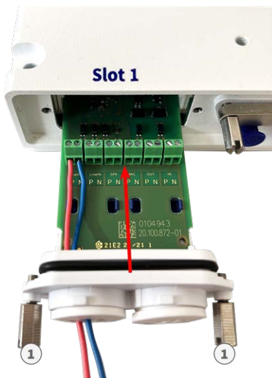
Fig. 23: Connecting the S74 Network Slide in Board with RJ45 socket
