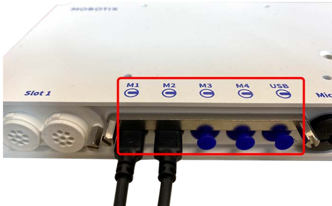
Fig. 22: 4 Module Connector Ports and 1 USB-C interface
