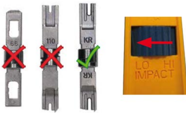
Fig. 12: LSA+/Krone tool set to LOW impact
