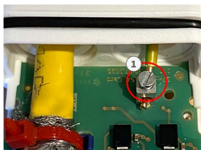
Fig. 15: Ground wire connected to terminal
